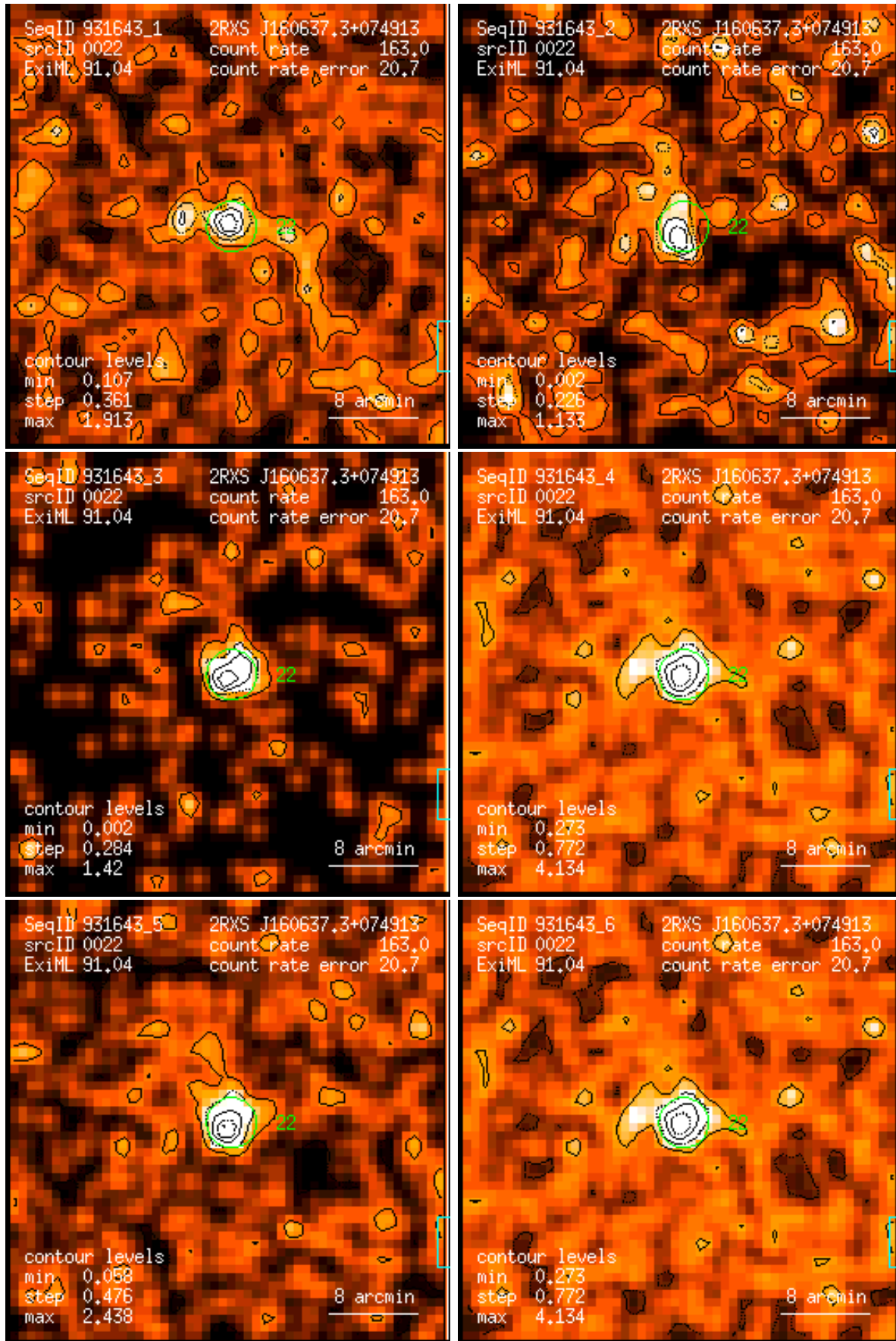
Figure 22: RASS 931643: detection 0022: band rate images, Gaussian filter: (1) PSPC channels 11 – 41, (2) 52 – 90, (3) 91 – 201, (4) 11 – 235, (5) 52 – 201, (6) 11 – 201. Broad band rates in counts/ks. Band rate contour levels in counts/ks/arcmin 2 .
