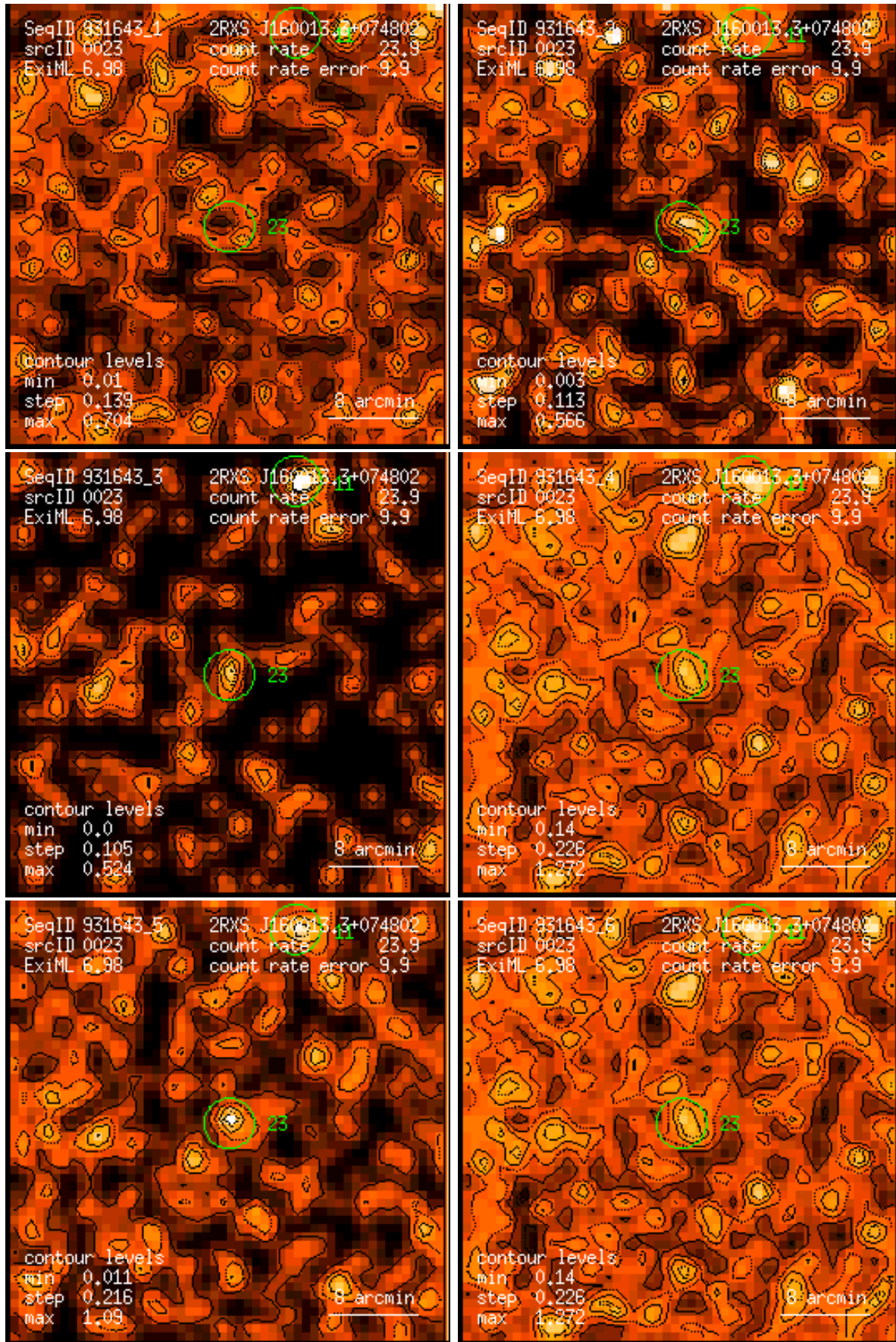
Figure 23: RASS 931643: detection 0023: band rate images, Gaussian filter: (1) PSPC channels 11 – 41, (2) 52 – 90, (3) 91 – 201, (4) 11 – 235, (5) 52 – 201, (6) 11 – 201. Broad band rates in counts/ks. Band rate contour levels in counts/ks/arcmin 2 .
