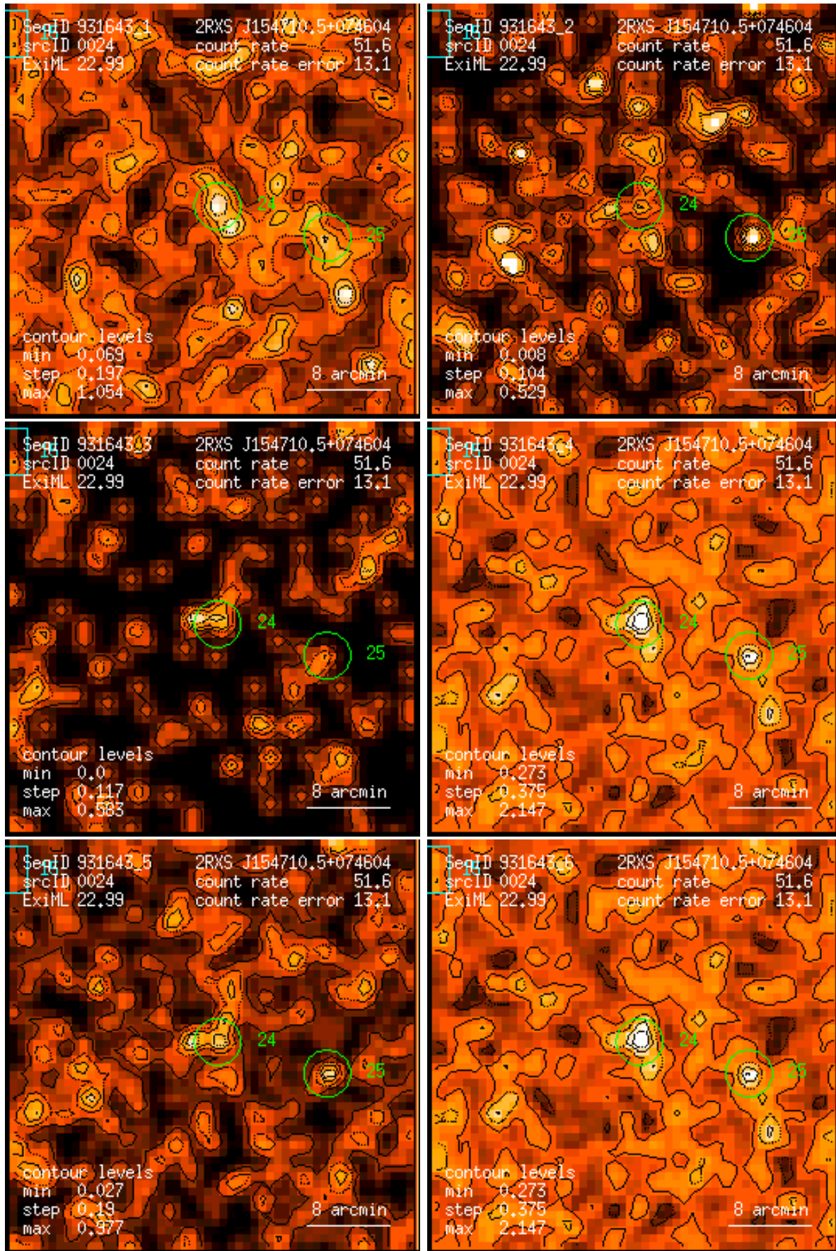
Figure 24: RASS 931643: detection 0024: band rate images, Gaussian filter: (1) PSPC channels 11 – 41, (2) 52 – 90, (3) 91 – 201, (4) 11 – 235, (5) 52 – 201, (6) 11 – 201. Broad band rates in counts/ks. Band rate contour levels in counts/ks/arcmin 2 .
