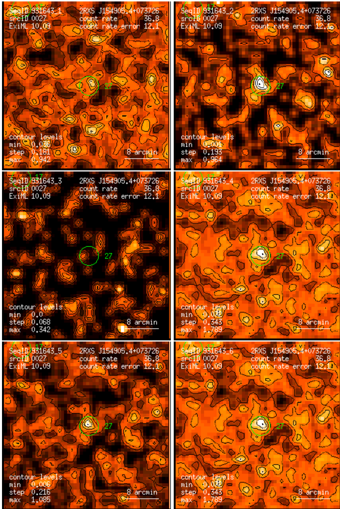
Figure 27: RASS 931643: detection 0027: band rate images, Gaussian filter: (1) PSPC channels 11 – 41, (2) 52 – 90, (3) 91 – 201, (4) 11 – 235, (5) 52 – 201, (6) 11 – 201. Broad band rates in counts/ks. Band rate contour levels in counts/ks/arcmin 2 .
