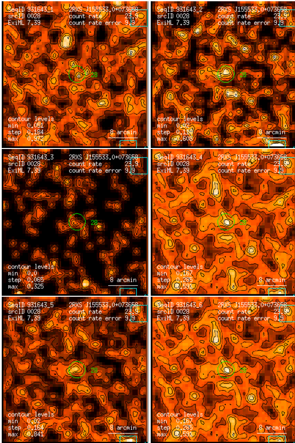
Figure 28: RASS 931643: detection 0028: band rate images, Gaussian filter: (1) PSPC channels 11 – 41, (2) 52 – 90, (3) 91 – 201, (4) 11 – 235, (5) 52 – 201, (6) 11 – 201. Broad band rates in counts/ks. Band rate contour levels in counts/ks/arcmin 2 .
