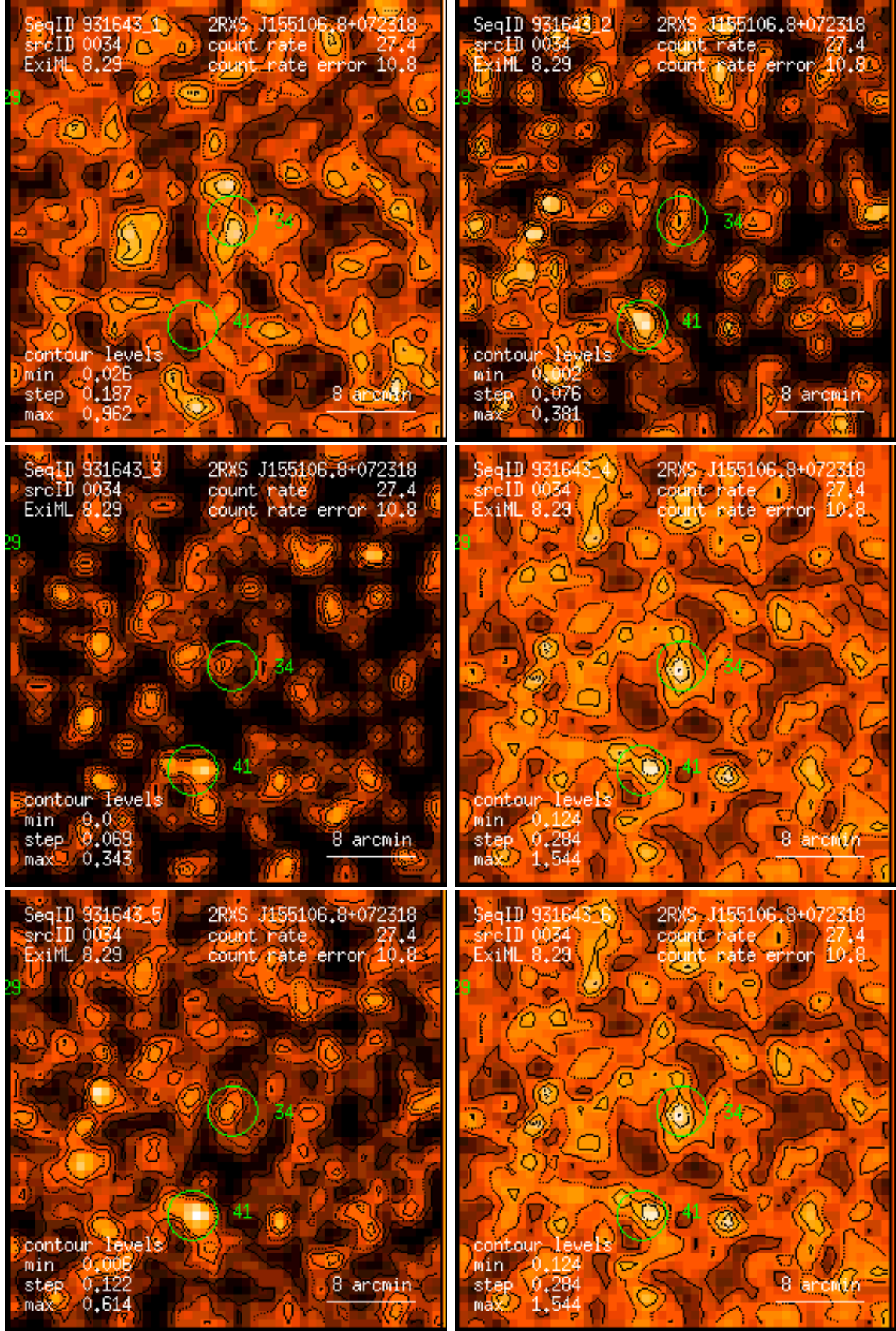
Figure 34: RASS 931643: detection 0034: band rate images, Gaussian filter: (1) PSPC channels 11 – 41, (2) 52 – 90, (3) 91 – 201, (4) 11 – 235, (5) 52 – 201, (6) 11 – 201. Broad band rates in counts/ks. Band rate contour levels in counts/ks/arcmin 2 .
