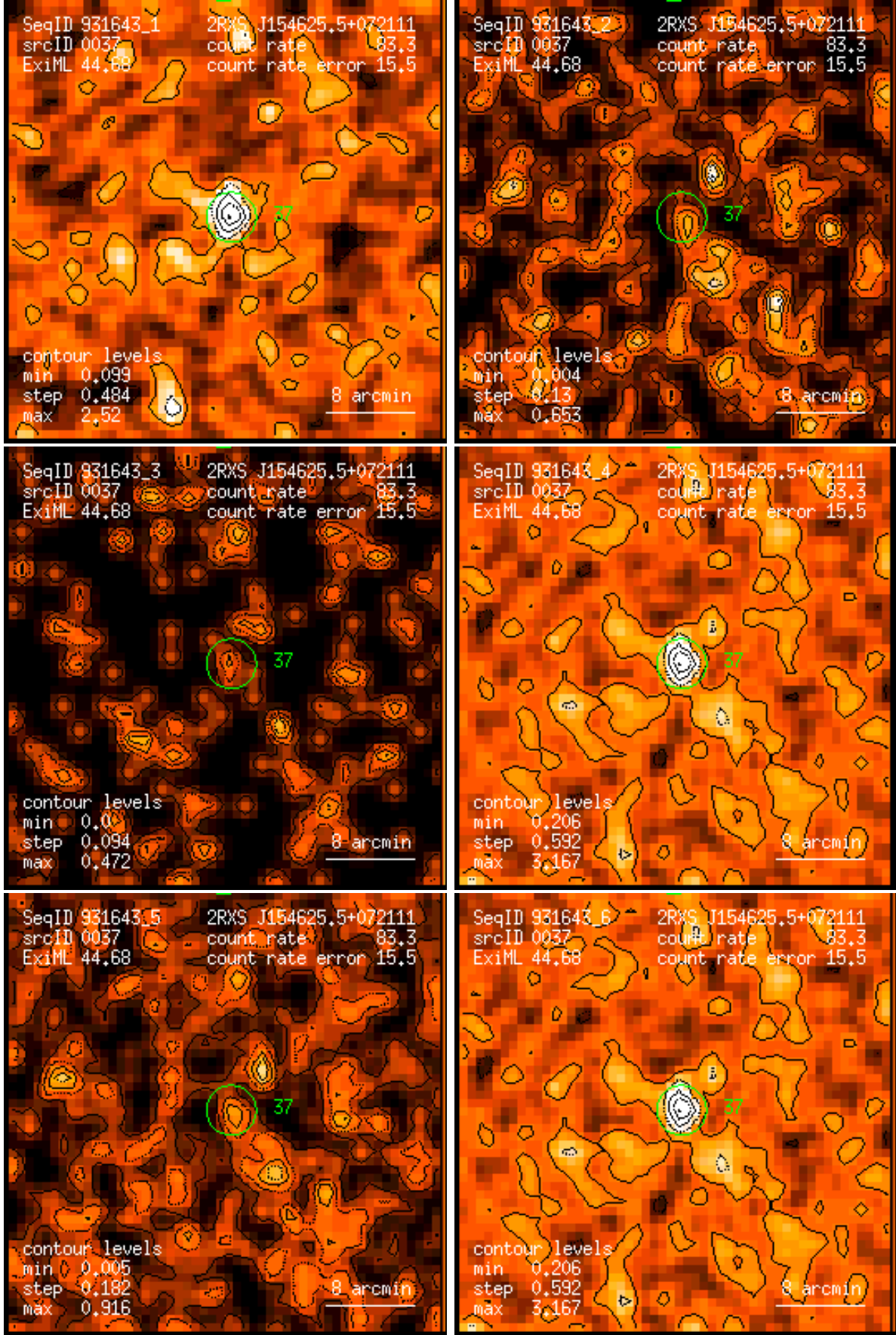
Figure 37: RASS 931643: detection 0037: band rate images, Gaussian filter: (1) PSPC channels 11 – 41, (2) 52 – 90, (3) 91 – 201, (4) 11 – 235, (5) 52 – 201, (6) 11 – 201. Broad band rates in counts/ks. Band rate contour levels in counts/ks/arcmin 2 .
