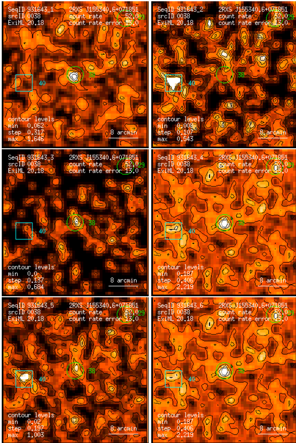
Figure 38: RASS 931643: detection 0038: band rate images, Gaussian filter: (1) PSPC channels 11 – 41, (2) 52 – 90, (3) 91 – 201, (4) 11 – 235, (5) 52 – 201, (6) 11 – 201. Broad band rates in counts/ks. Band rate contour levels in counts/ks/arcmin 2 .
