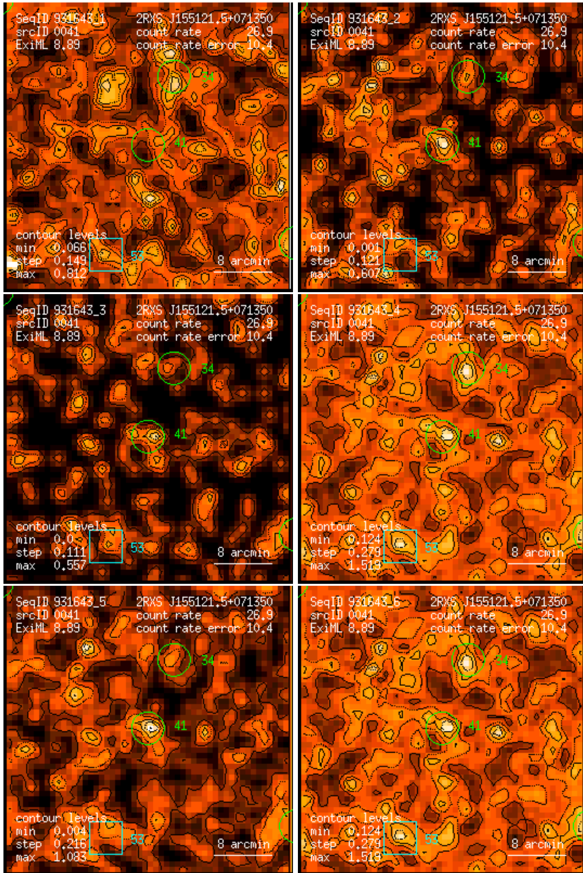
Figure 41: RASS 931643: detection 0041: band rate images, Gaussian filter: (1) PSPC channels 11 – 41, (2) 52 – 90, (3) 91 – 201, (4) 11 – 235, (5) 52 – 201, (6) 11 – 201. Broad band rates in counts/ks. Band rate contour levels in counts/ks/arcmin 2 .
