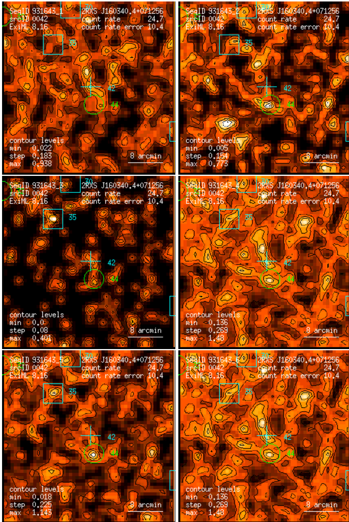
Figure 42: RASS 931643: detection 0042: band rate images, Gaussian filter: (1) PSPC channels 11 – 41, (2) 52 – 90, (3) 91 – 201, (4) 11 – 235, (5) 52 – 201, (6) 11 – 201. Broad band rates in counts/ks. Band rate contour levels in counts/ks/arcmin 2 .
