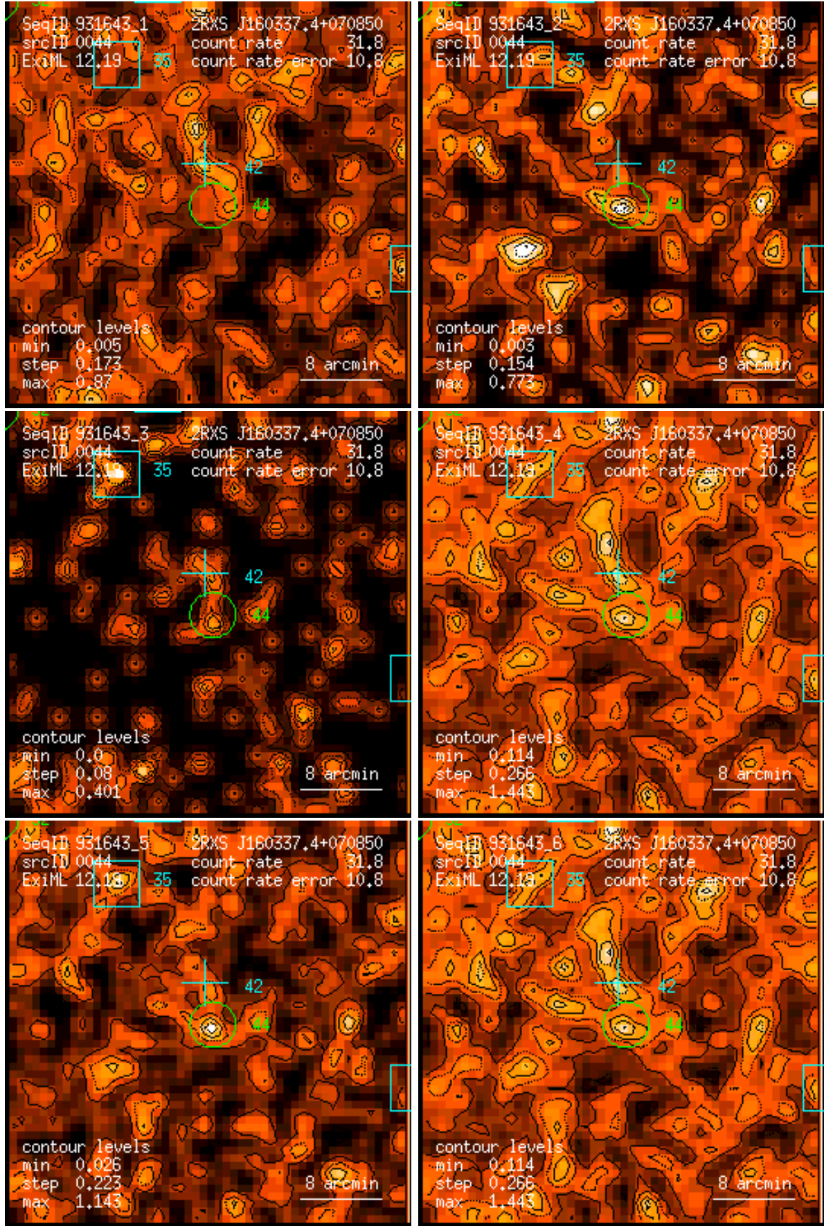
Figure 44: RASS 931643: detection 0044: band rate images, Gaussian filter: (1) PSPC channels 11 – 41, (2) 52 – 90, (3) 91 – 201, (4) 11 – 235, (5) 52 – 201, (6) 11 – 201. Broad band rates in counts/ks. Band rate contour levels in counts/ks/arcmin 2 .
