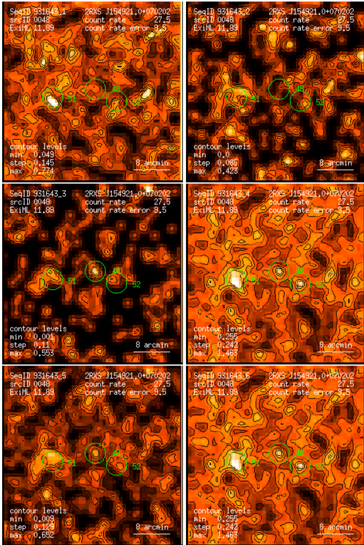
Figure 48: RASS 931643: detection 0048: band rate images, Gaussian filter: (1) PSPC channels 11 – 41, (2) 52 – 90, (3) 91 – 201, (4) 11 – 235, (5) 52 – 201, (6) 11 – 201. Broad band rates in counts/ks. Band rate contour levels in counts/ks/arcmin 2 .
