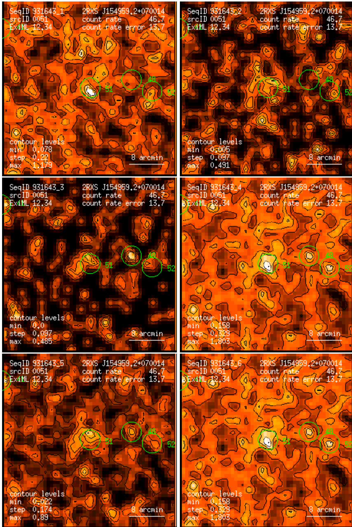
Figure 51: RASS 931643: detection 0051: band rate images, Gaussian filter: (1) PSPC channels 11 – 41, (2) 52 – 90, (3) 91 – 201, (4) 11 – 235, (5) 52 – 201, (6) 11 – 201. Broad band rates in counts/ks. Band rate contour levels in counts/ks/arcmin 2 .
