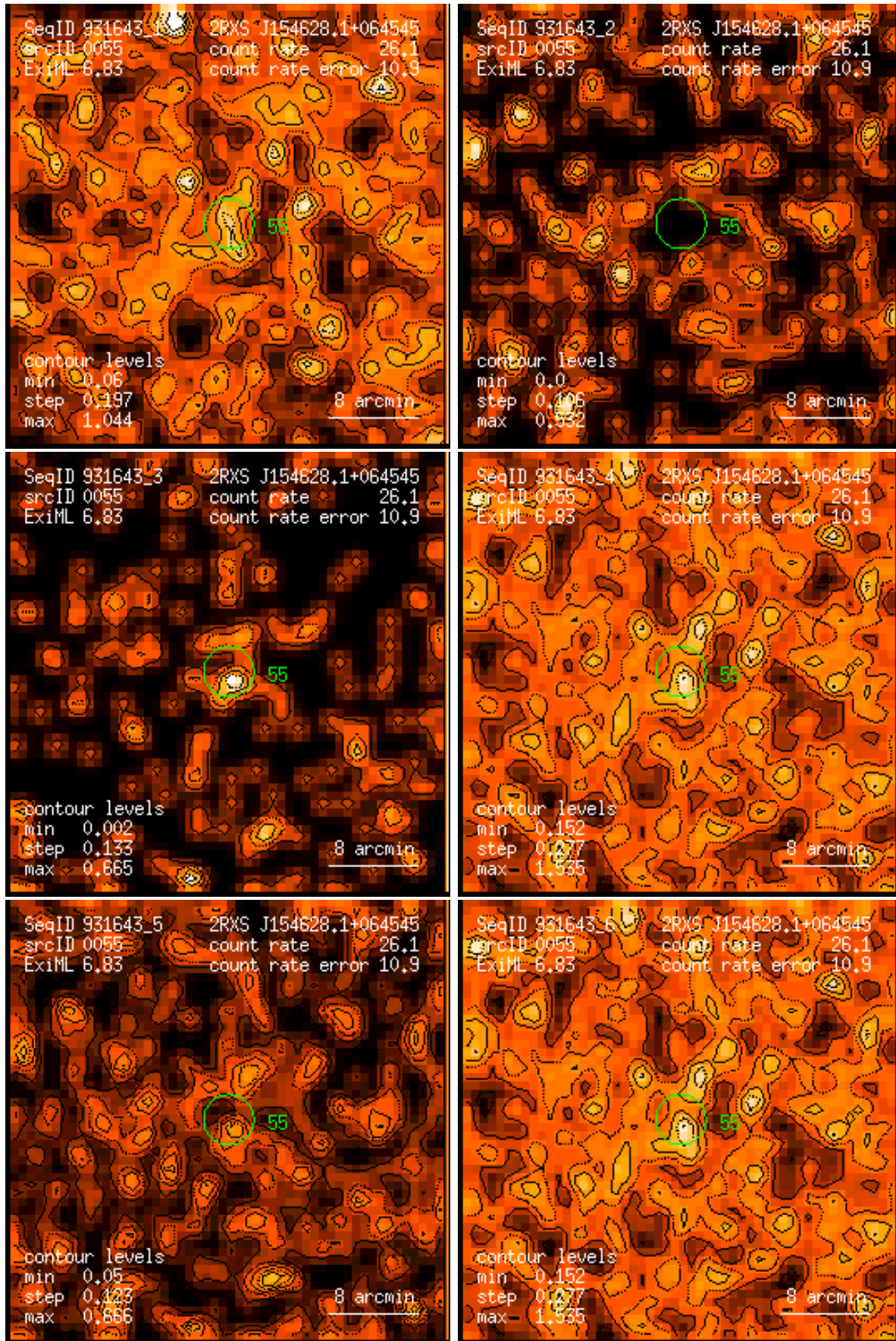
Figure 55: RASS 931643: detection 0055: band rate images, Gaussian filter: (1) PSPC channels 11 – 41, (2) 52 – 90, (3) 91 – 201, (4) 11 – 235, (5) 52 – 201, (6) 11 – 201. Broad band rates in counts/ks. Band rate contour levels in counts/ks/arcmin 2 .
