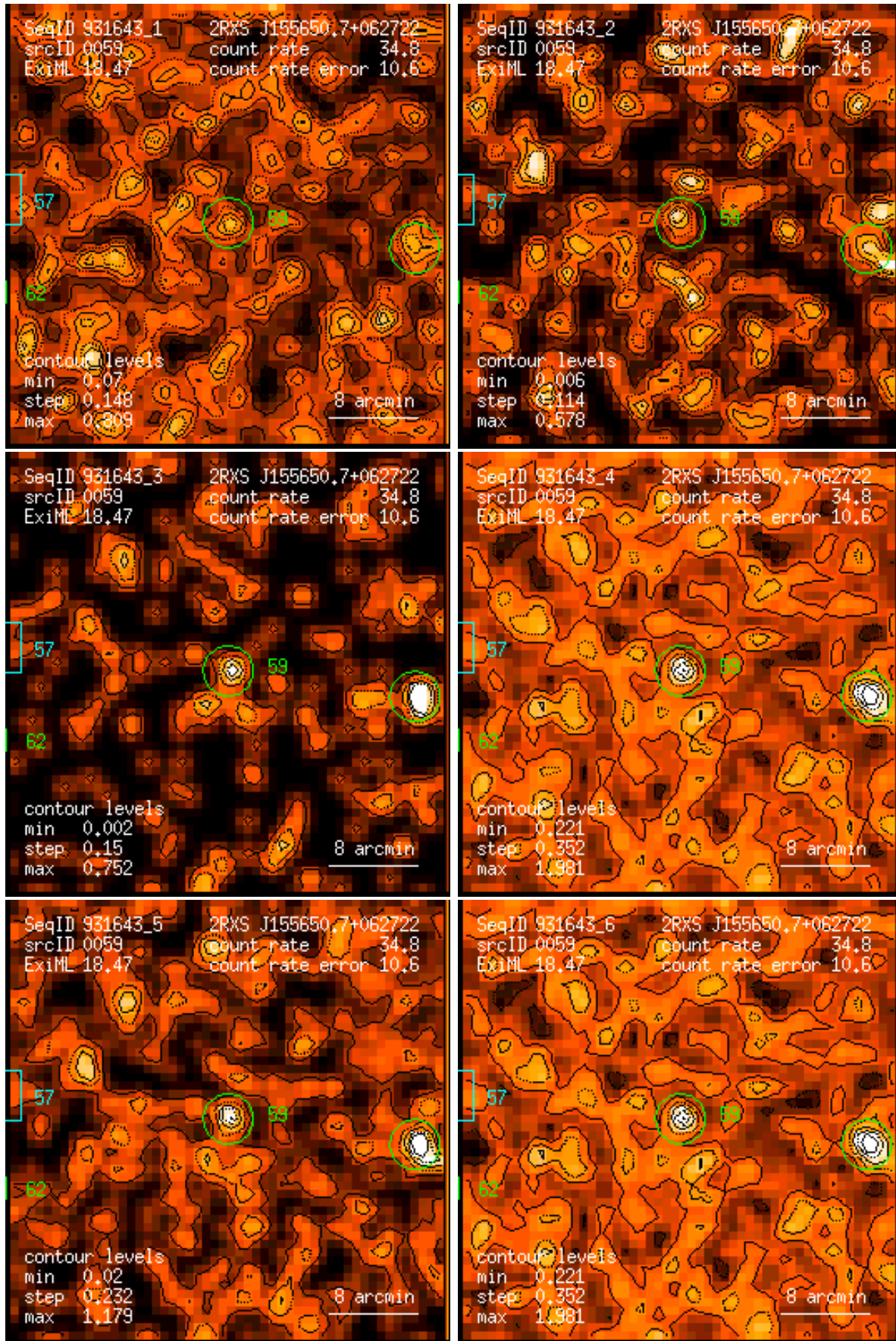
Figure 59: RASS 931643: detection 0059: band rate images, Gaussian filter: (1) PSPC channels 11 – 41, (2) 52 – 90, (3) 91 – 201, (4) 11 – 235, (5) 52 – 201, (6) 11 – 201. Broad band rates in counts/ks. Band rate contour levels in counts/ks/arcmin 2 .
