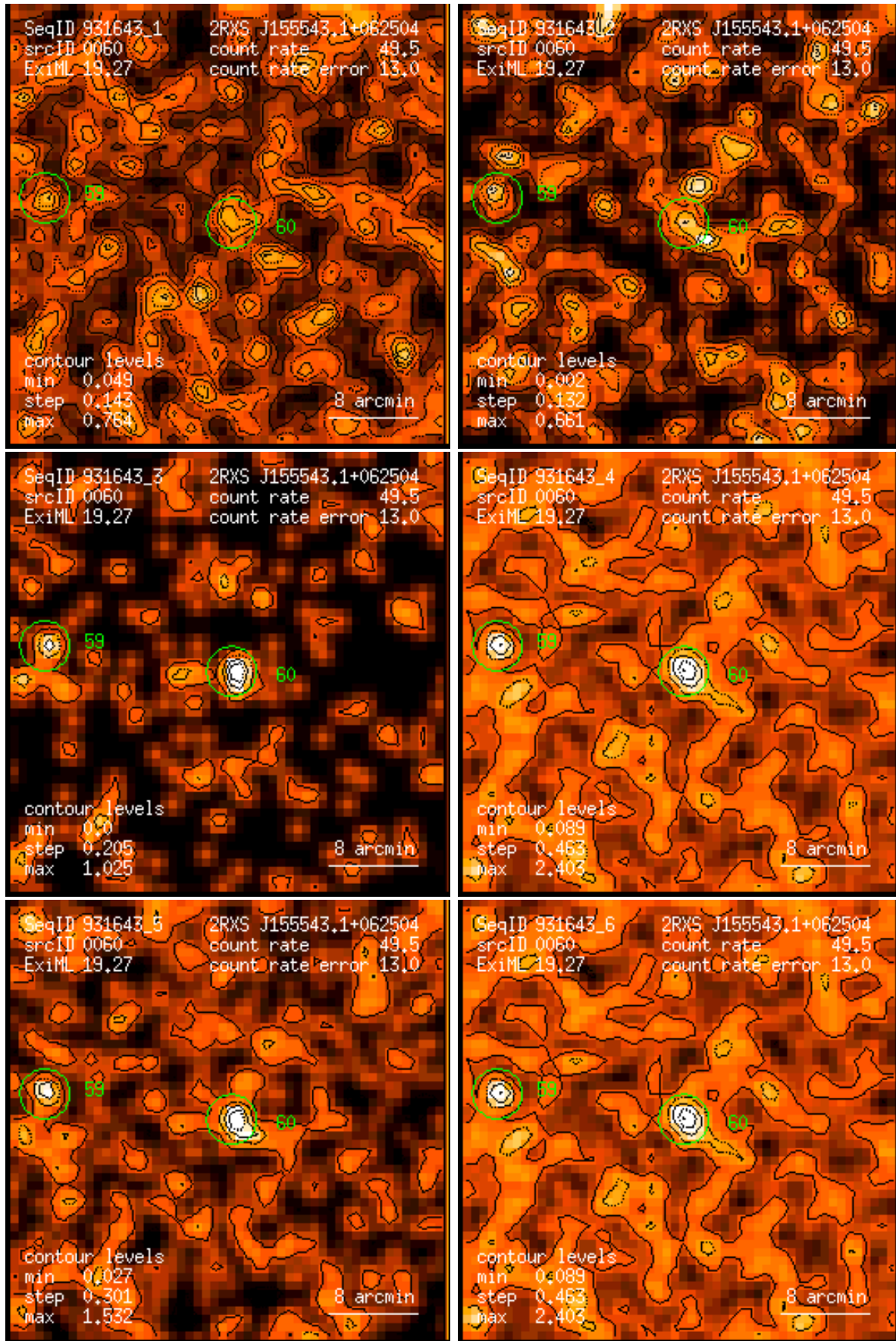
Figure 60: RASS 931643: detection 0060: band rate images, Gaussian filter: (1) PSPC channels 11 – 41, (2) 52 – 90, (3) 91 – 201, (4) 11 – 235, (5) 52 – 201, (6) 11 – 201. Broad band rates in counts/ks. Band rate contour levels in counts/ks/arcmin 2 .
