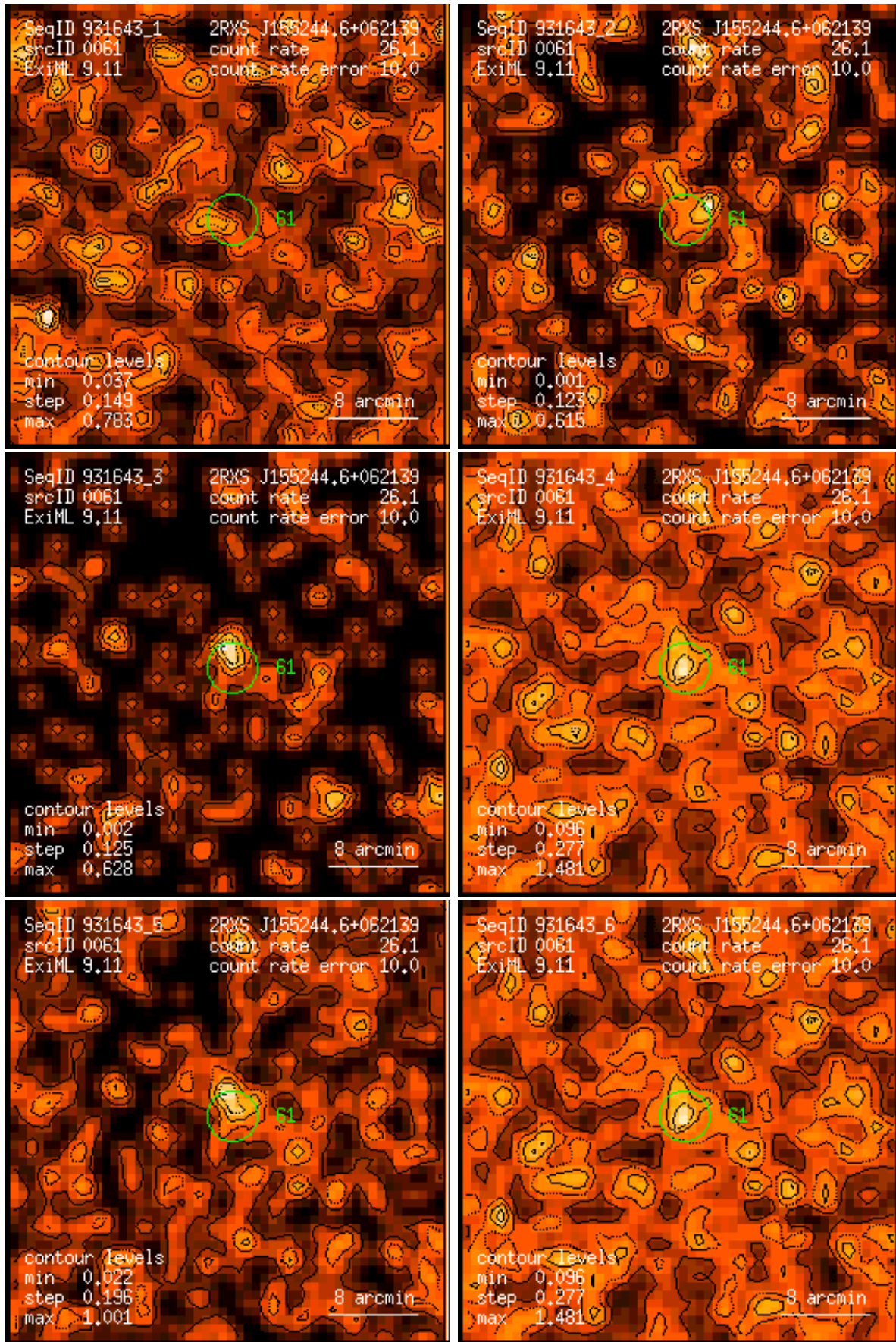
Figure 61: RASS 931643: detection 0061: band rate images, Gaussian filter: (1) PSPC channels 11 – 41, (2) 52 – 90, (3) 91 – 201, (4) 11 – 235, (5) 52 – 201, (6) 11 – 201. Broad band rates in counts/ks. Band rate contour levels in counts/ks/arcmin 2 .
