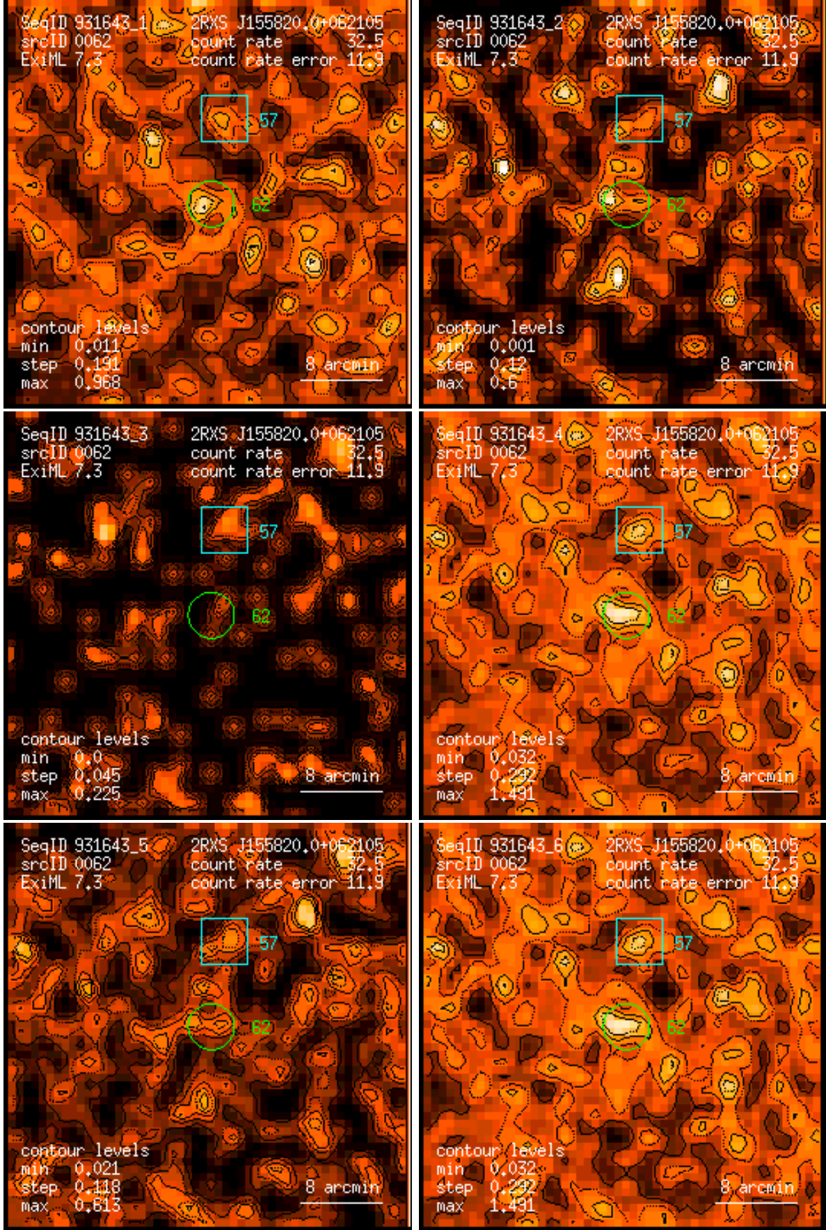
Figure 62: RASS 931643: detection 0062: band rate images, Gaussian filter: (1) PSPC channels 11 – 41, (2) 52 – 90, (3) 91 – 201, (4) 11 – 235, (5) 52 – 201, (6) 11 – 201. Broad band rates in counts/ks. Band rate contour levels in counts/ks/arcmin 2 .
