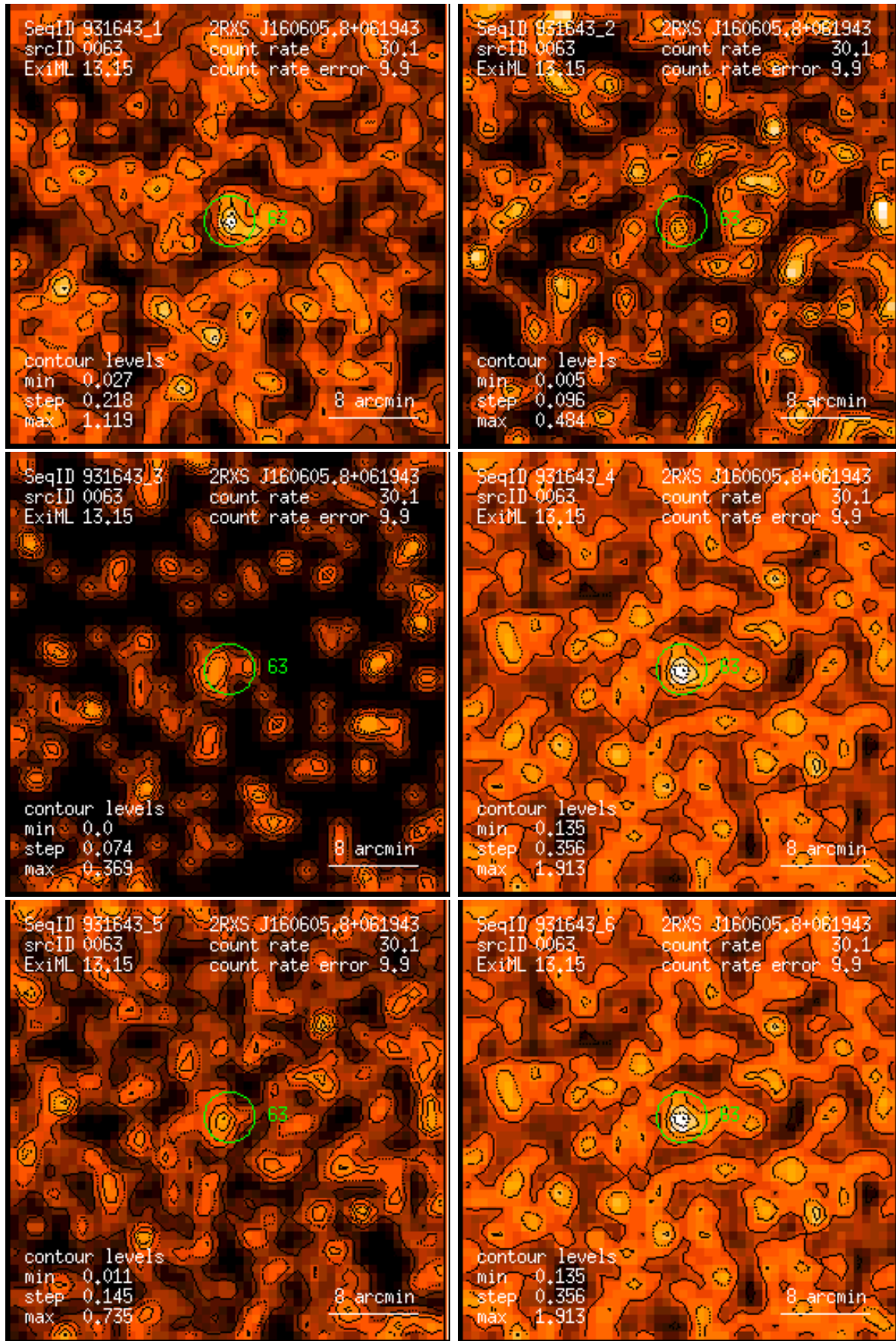
Figure 63: RASS 931643: detection 0063: band rate images, Gaussian filter: (1) PSPC channels 11 – 41, (2) 52 – 90, (3) 91 – 201, (4) 11 – 235, (5) 52 – 201, (6) 11 – 201. Broad band rates in counts/ks. Band rate contour levels in counts/ks/arcmin 2 .
