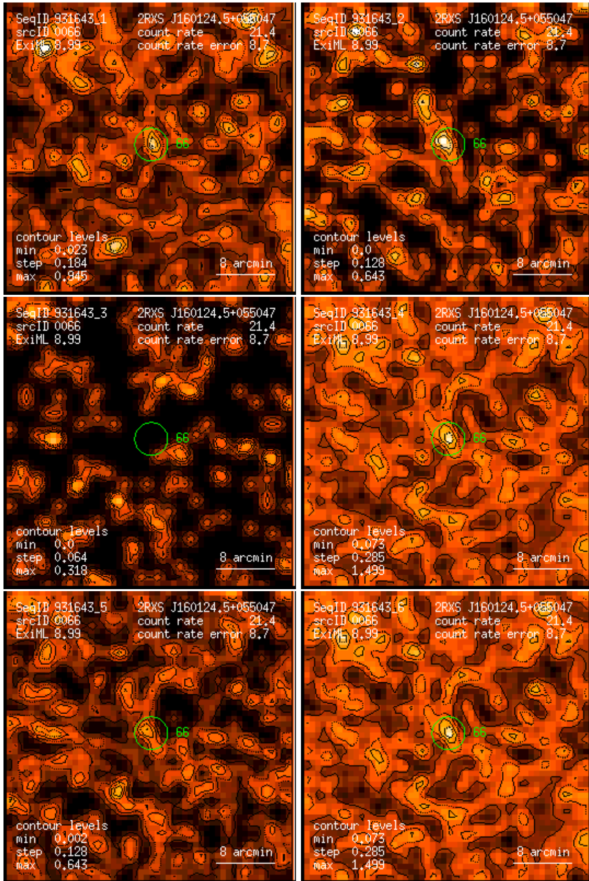
Figure 66: RASS 931643: detection 0066: band rate images, Gaussian filter: (1) PSPC channels 11 – 41, (2) 52 – 90, (3) 91 – 201, (4) 11 – 235, (5) 52 – 201, (6) 11 – 201. Broad band rates in counts/ks. Band rate contour levels in counts/ks/arcmin 2 .
