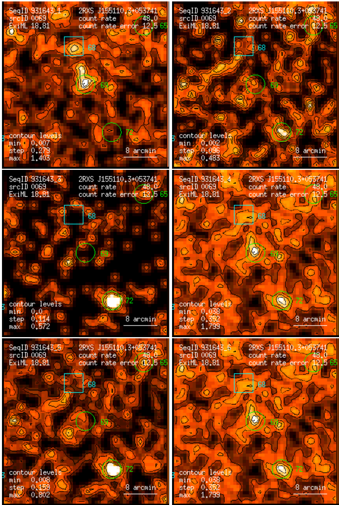
Figure 69: RASS 931643: detection 0069: band rate images, Gaussian filter: (1) PSPC channels 11 – 41, (2) 52 – 90, (3) 91 – 201, (4) 11 – 235, (5) 52 – 201, (6) 11 – 201. Broad band rates in counts/ks. Band rate contour levels in counts/ks/arcmin 2 .
