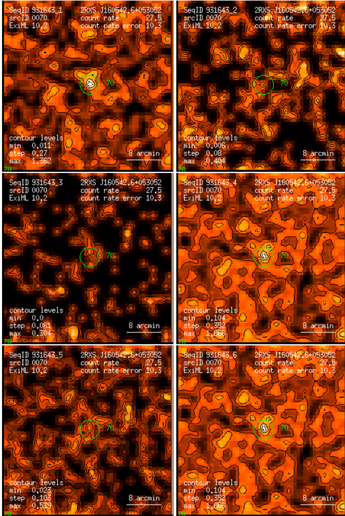
Figure 70: RASS 931643: detection 0070: band rate images, Gaussian filter: (1) PSPC channels 11 – 41, (2) 52 – 90, (3) 91 – 201, (4) 11 – 235, (5) 52 – 201, (6) 11 – 201. Broad band rates in counts/ks. Band rate contour levels in counts/ks/arcmin 2 .
