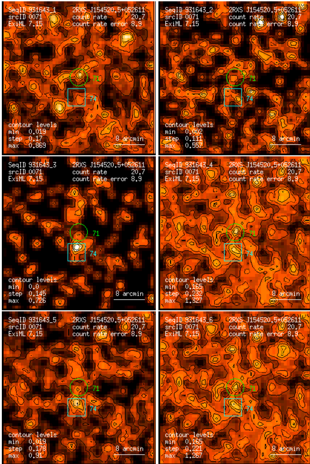
Figure 71: RASS 931643: detection 0071: band rate images, Gaussian filter: (1) PSPC channels 11 – 41, (2) 52 – 90, (3) 91 – 201, (4) 11 – 235, (5) 52 – 201, (6) 11 – 201. Broad band rates in counts/ks. Band rate contour levels in counts/ks/arcmin 2 .
