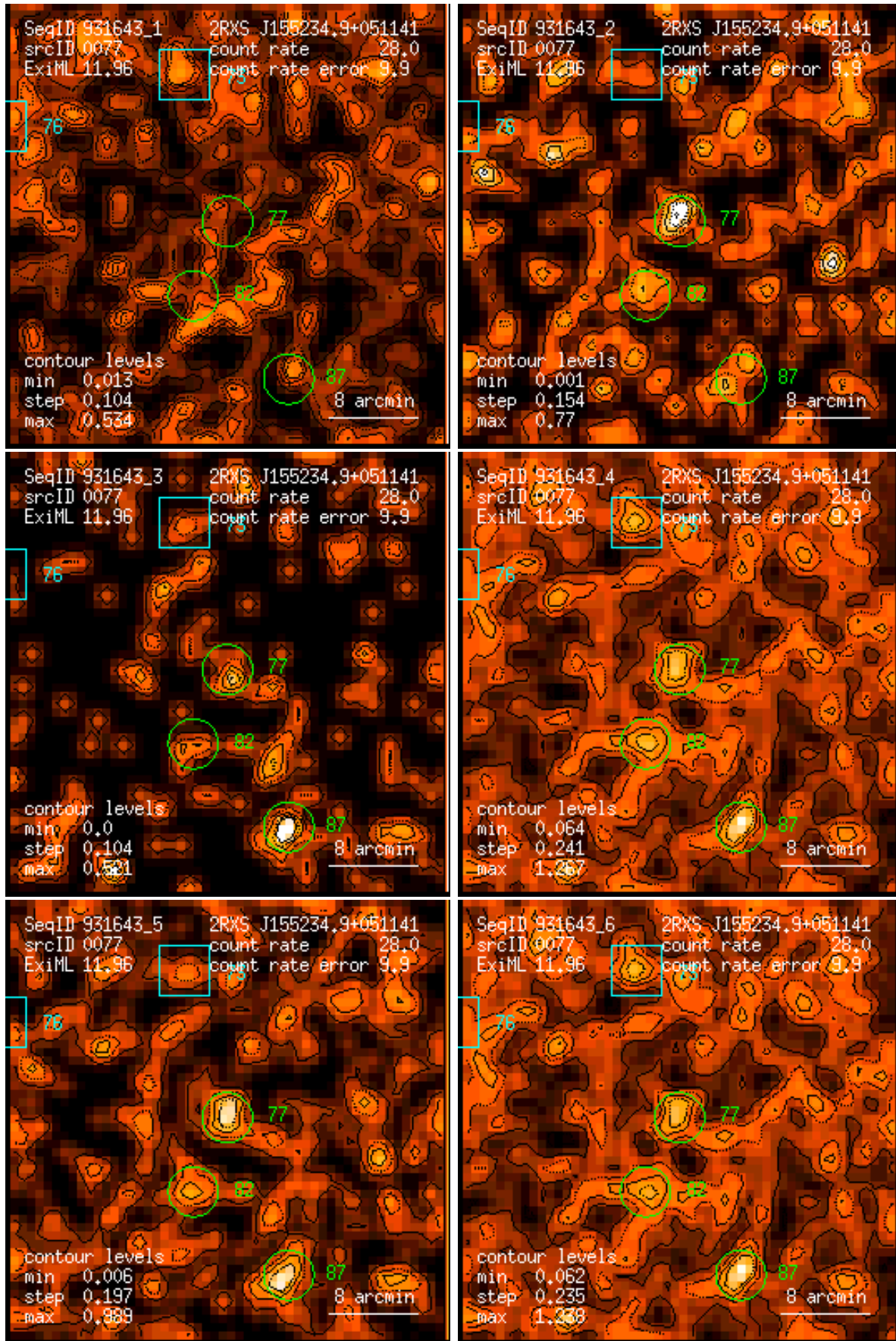
Figure 77: RASS 931643: detection 0077: band rate images, Gaussian filter: (1) PSPC channels 11 – 41, (2) 52 – 90, (3) 91 – 201, (4) 11 – 235, (5) 52 – 201, (6) 11 – 201. Broad band rates in counts/ks. Band rate contour levels in counts/ks/arcmin 2 .
