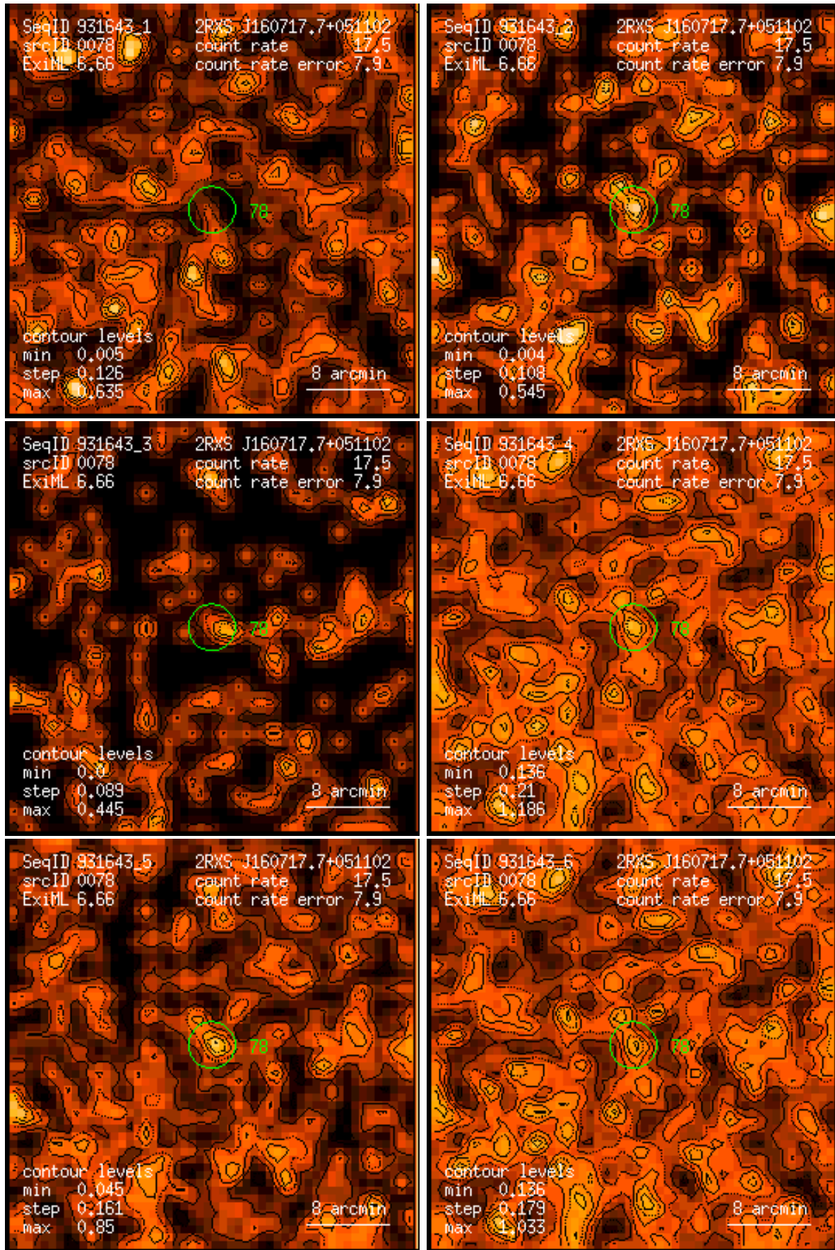
Figure 78: RASS 931643: detection 0078: band rate images, Gaussian filter: (1) PSPC channels 11 – 41, (2) 52 – 90, (3) 91 – 201, (4) 11 – 235, (5) 52 – 201, (6) 11 – 201. Broad band rates in counts/ks. Band rate contour levels in counts/ks/arcmin 2 .
