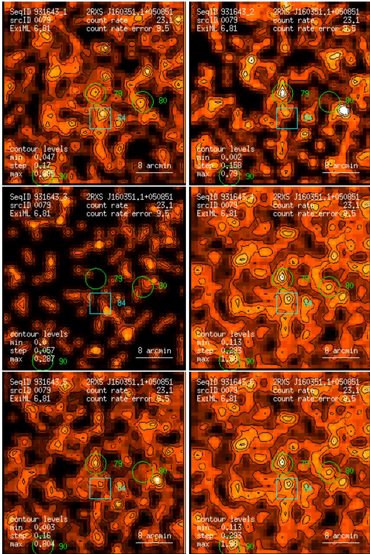
Figure 79: RASS 931643: detection 0079: band rate images, Gaussian filter: (1) PSPC channels 11 – 41, (2) 52 – 90, (3) 91 – 201, (4) 11 – 235, (5) 52 – 201, (6) 11 – 201. Broad band rates in counts/ks. Band rate contour levels in counts/ks/arcmin 2 .
