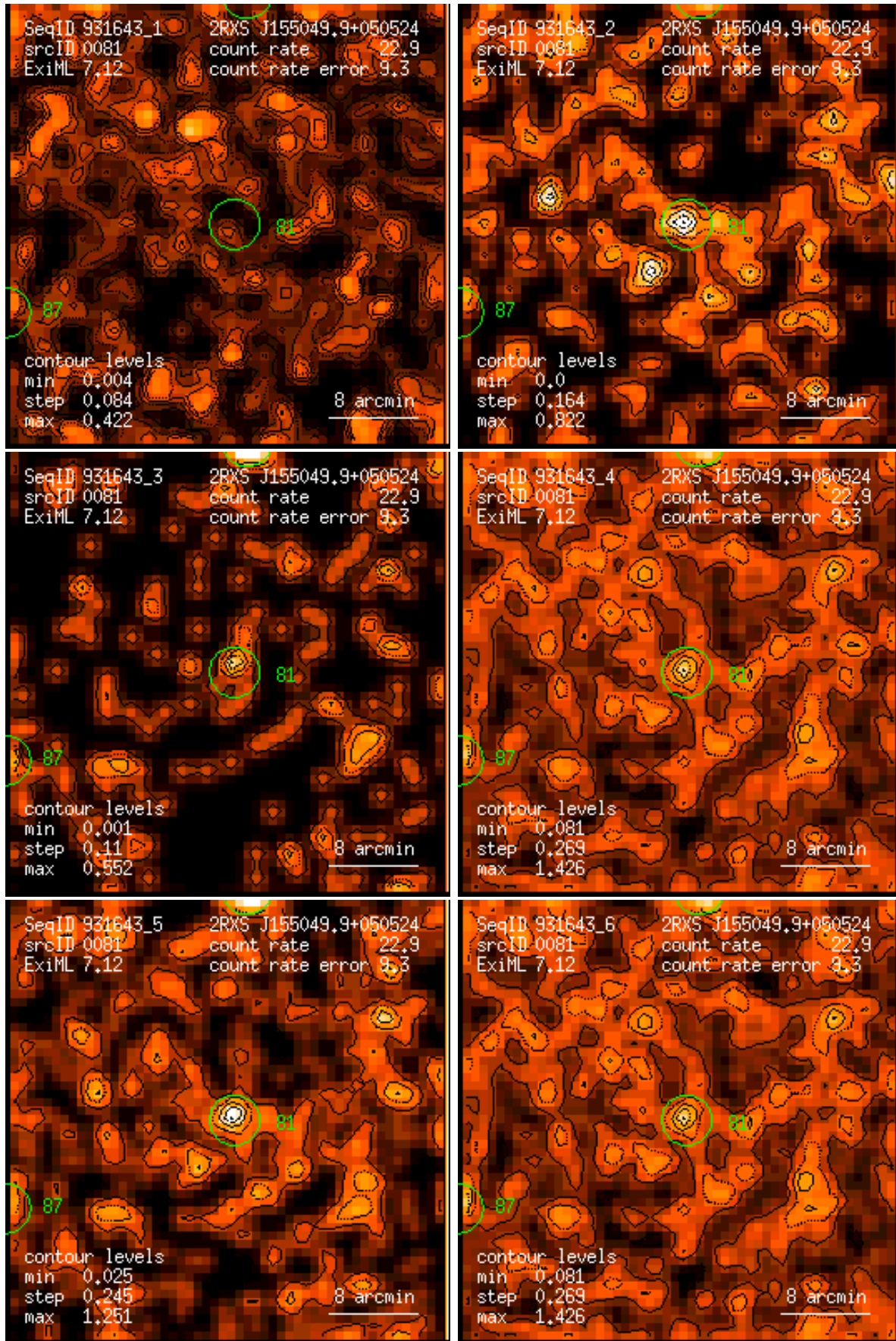
Figure 81: RASS 931643: detection 0081: band rate images, Gaussian filter: (1) PSPC channels 11 – 41, (2) 52 – 90, (3) 91 – 201, (4) 11 – 235, (5) 52 – 201, (6) 11 – 201. Broad band rates in counts/ks. Band rate contour levels in counts/ks/arcmin 2 .
