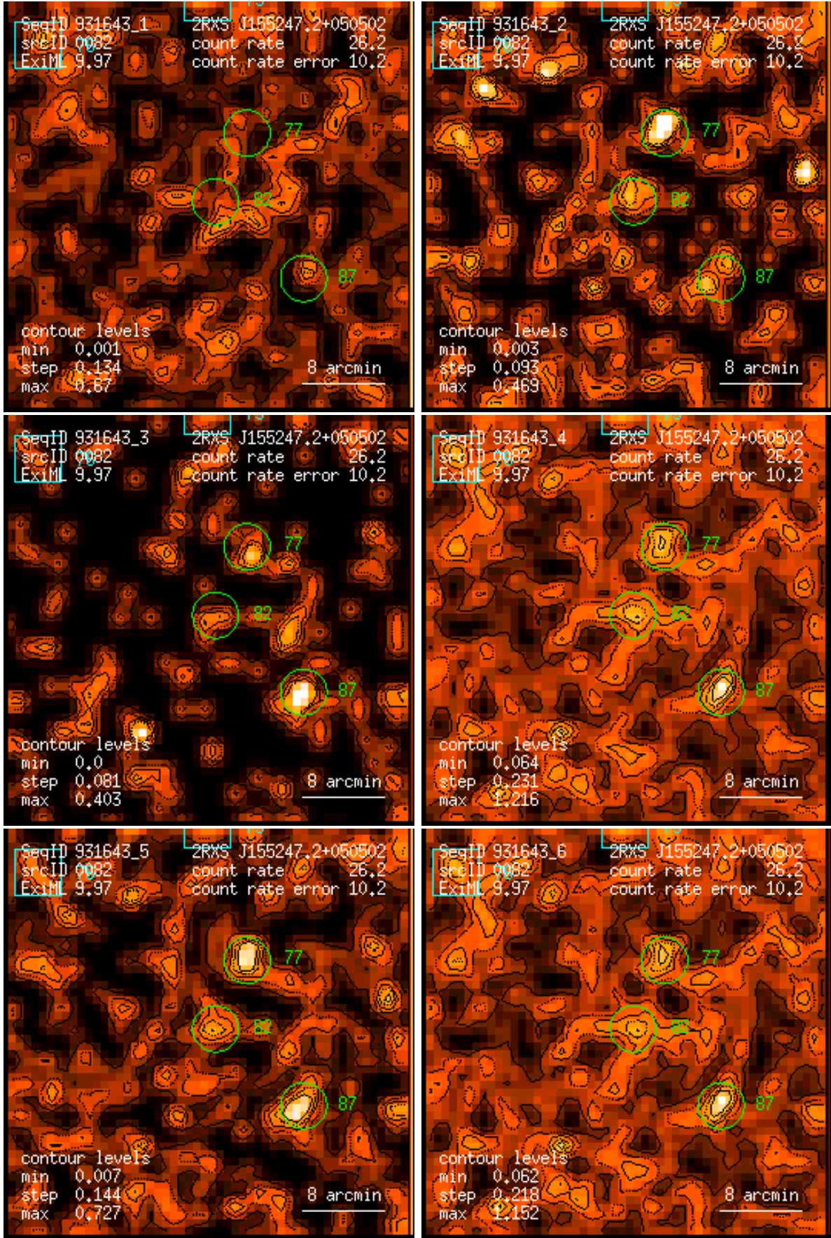
Figure 82: RASS 931643: detection 0082: band rate images, Gaussian filter: (1) PSPC channels 11 – 41, (2) 52 – 90, (3) 91 – 201, (4) 11 – 235, (5) 52 – 201, (6) 11 – 201. Broad band rates in counts/ks. Band rate contour levels in counts/ks/arcmin 2 .
