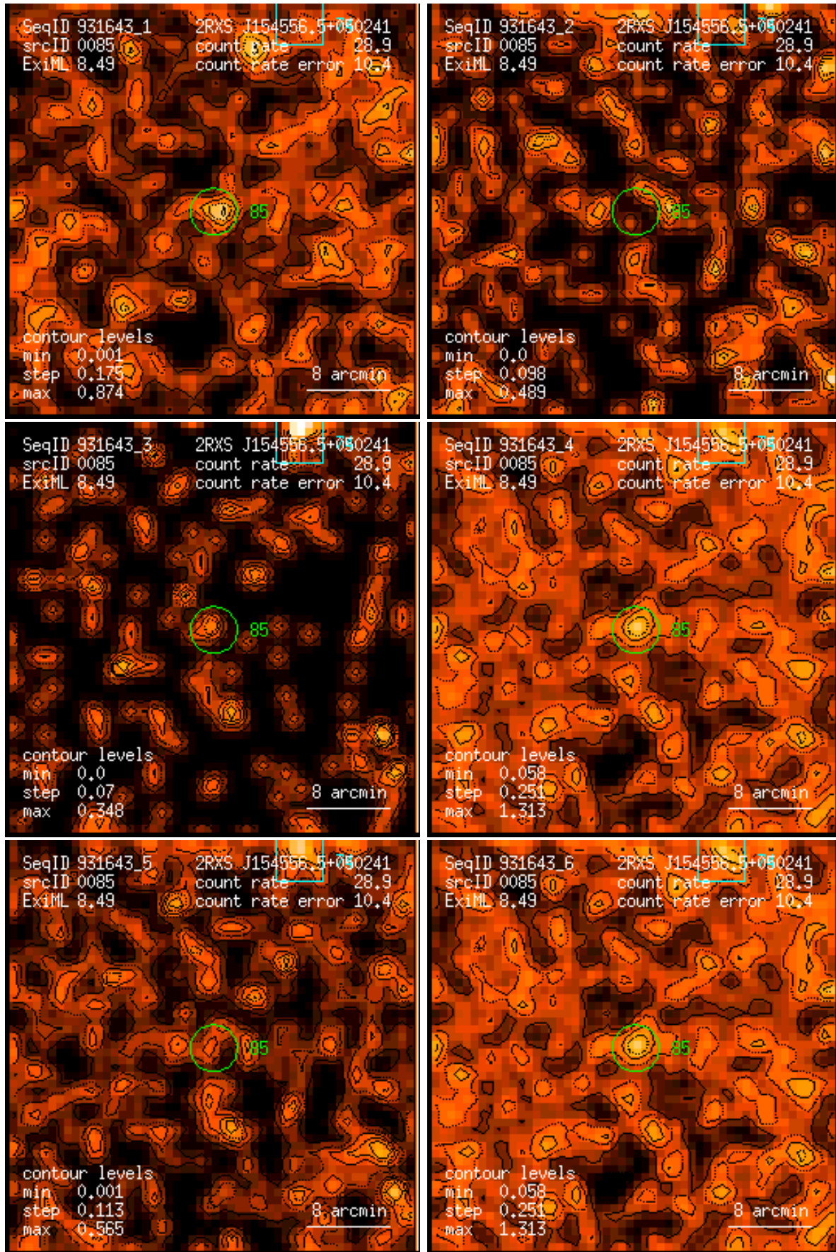
Figure 85: RASS 931643: detection 0085: band rate images, Gaussian filter: (1) PSPC channels 11 – 41, (2) 52 – 90, (3) 91 – 201, (4) 11 – 235, (5) 52 – 201, (6) 11 – 201. Broad band rates in counts/ks. Band rate contour levels in counts/ks/arcmin 2 .
