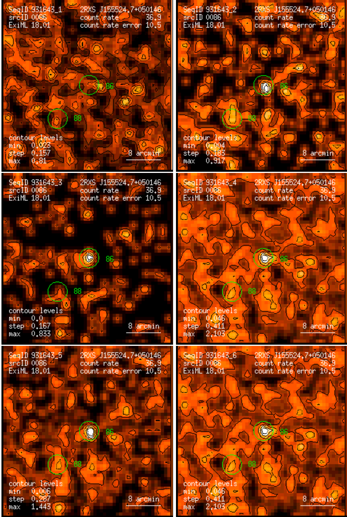
Figure 86: RASS 931643: detection 0086: band rate images, Gaussian filter: (1) PSPC channels 11 – 41, (2) 52 – 90, (3) 91 – 201, (4) 11 – 235, (5) 52 – 201, (6) 11 – 201. Broad band rates in counts/ks. Band rate contour levels in counts/ks/arcmin 2 .
