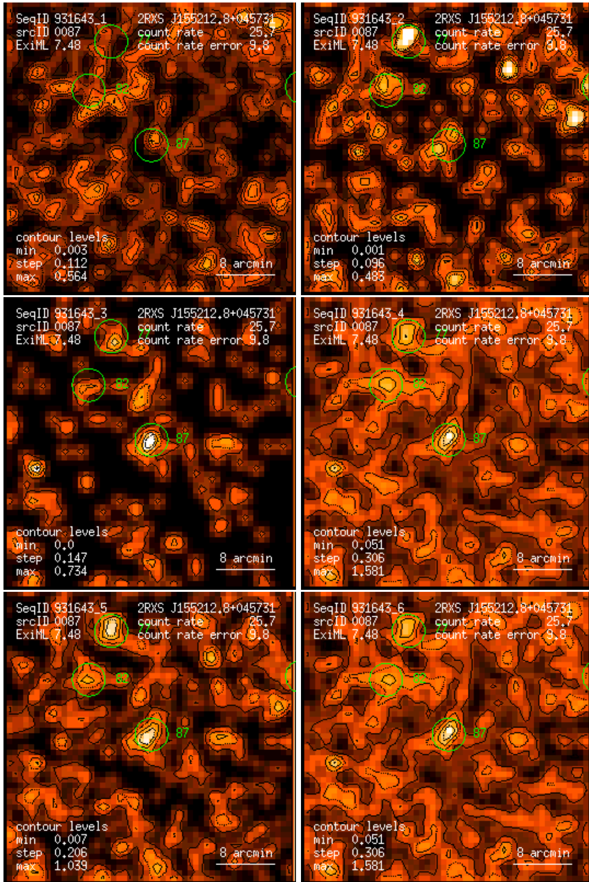
Figure 87: RASS 931643: detection 0087: band rate images, Gaussian filter: (1) PSPC channels 11 – 41, (2) 52 – 90, (3) 91 – 201, (4) 11 – 235, (5) 52 – 201, (6) 11 – 201. Broad band rates in counts/ks. Band rate contour levels in counts/ks/arcmin 2 .
