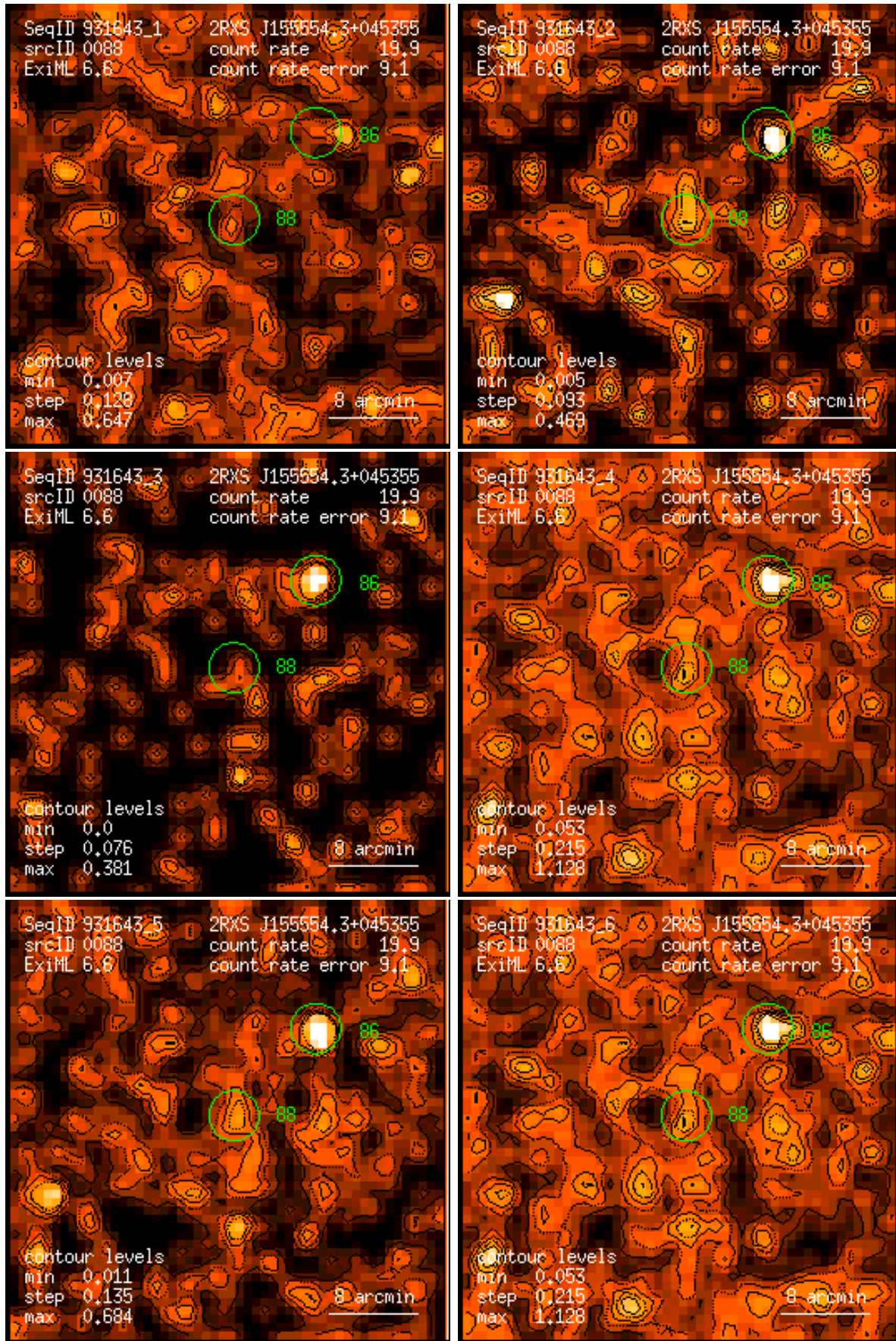
Figure 88: RASS 931643: detection 0088: band rate images, Gaussian filter: (1) PSPC channels 11 – 41, (2) 52 – 90, (3) 91 – 201, (4) 11 – 235, (5) 52 – 201, (6) 11 – 201. Broad band rates in counts/ks. Band rate contour levels in counts/ks/arcmin 2 .
