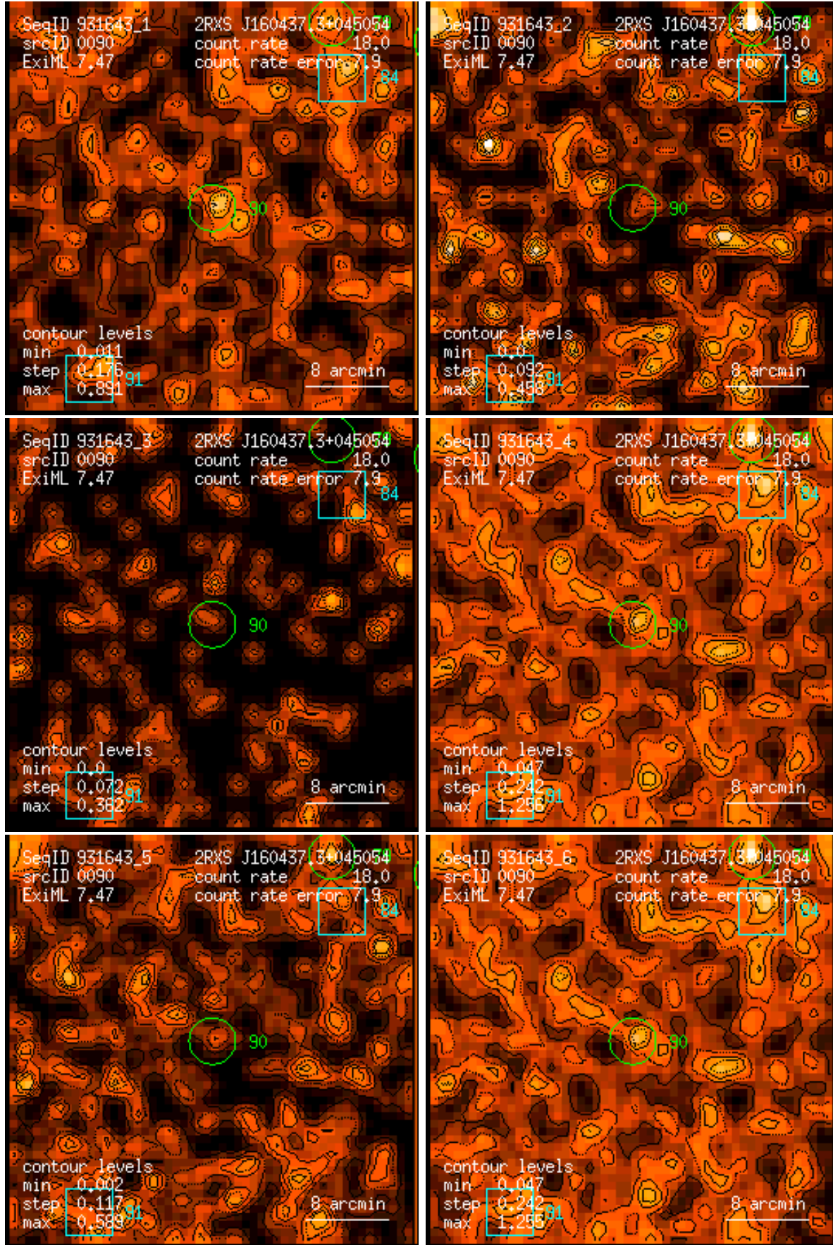
Figure 90: RASS 931643: detection 0090: band rate images, Gaussian filter: (1) PSPC channels 11 – 41, (2) 52 – 90, (3) 91 – 201, (4) 11 – 235, (5) 52 – 201, (6) 11 – 201. Broad band rates in counts/ks. Band rate contour levels in counts/ks/arcmin 2 .
