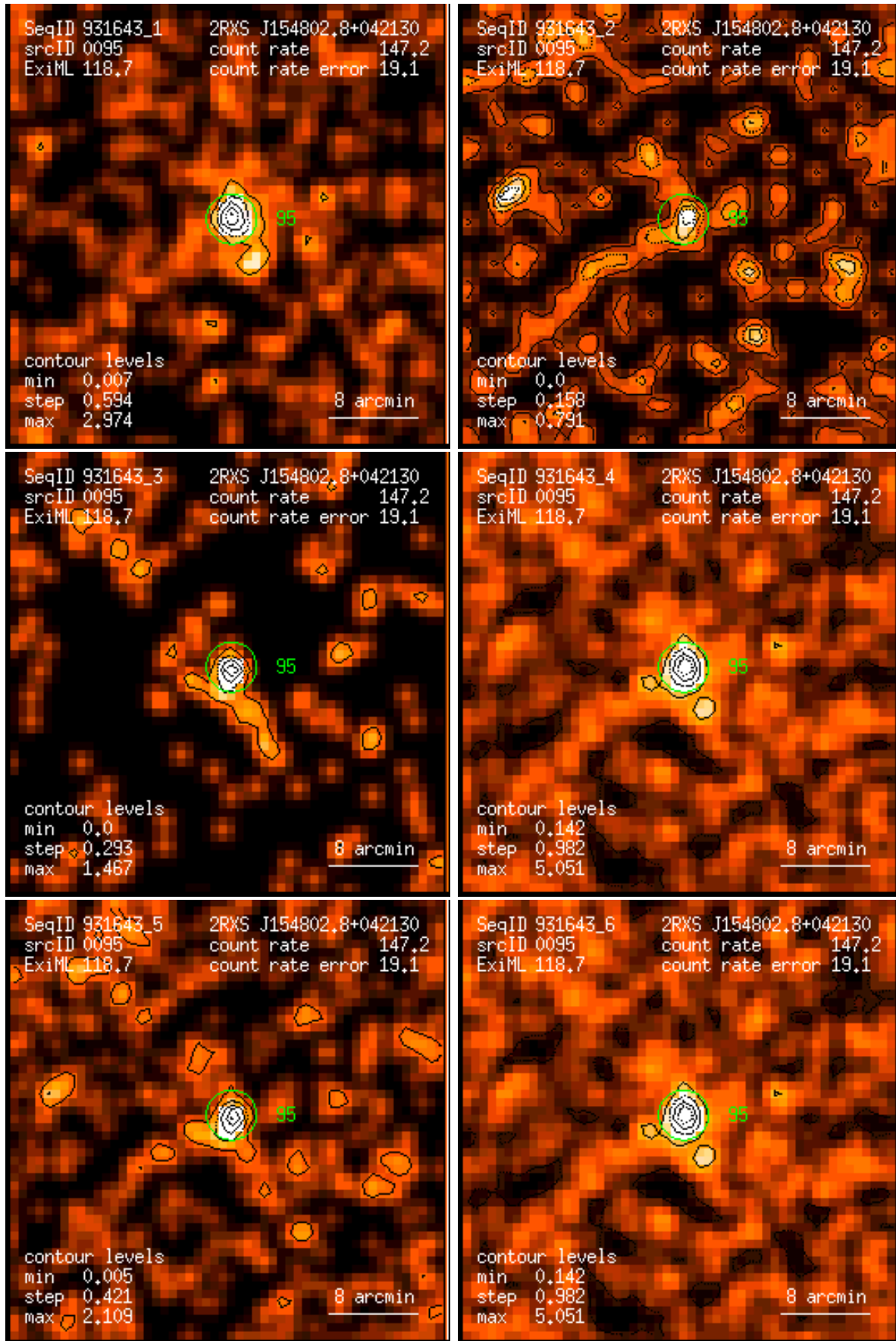
Figure 95: RASS 931643: detection 0095: band rate images, Gaussian filter: (1) PSPC channels 11 – 41, (2) 52 – 90, (3) 91 – 201, (4) 11 – 235, (5) 52 – 201, (6) 11 – 201. Broad band rates in counts/ks. Band rate contour levels in counts/ks/arcmin 2 .
