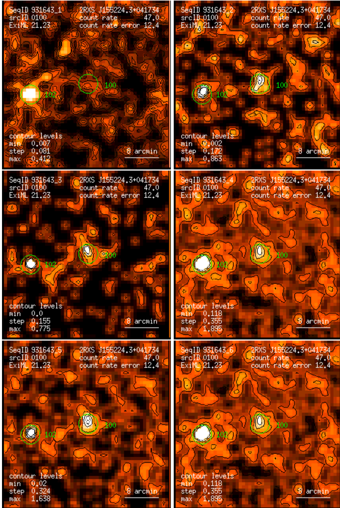
Figure 100: RASS 931643: detection 0100: band rate images, Gaussian filter: (1) PSPC channels 11 – 41, (2) 52 – 90, (3) 91 – 201, (4) 11 – 235, (5) 52 – 201, (6) 11 – 201. Broad band rates in counts/ks. Band rate contour levels in counts/ks/arcmin 2 .
