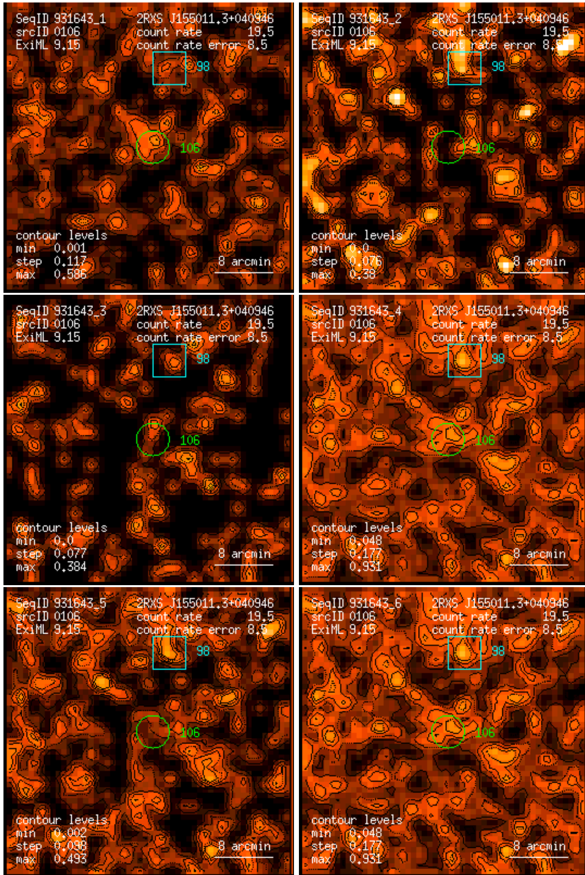
Figure 106: RASS 931643: detection 0106: band rate images, Gaussian filter: (1) PSPC channels 11 – 41, (2) 52 – 90, (3) 91 – 201, (4) 11 – 235, (5) 52 – 201, (6) 11 – 201. Broad band rates in counts/ks. Band rate contour levels in counts/ks/arcmin 2 .
