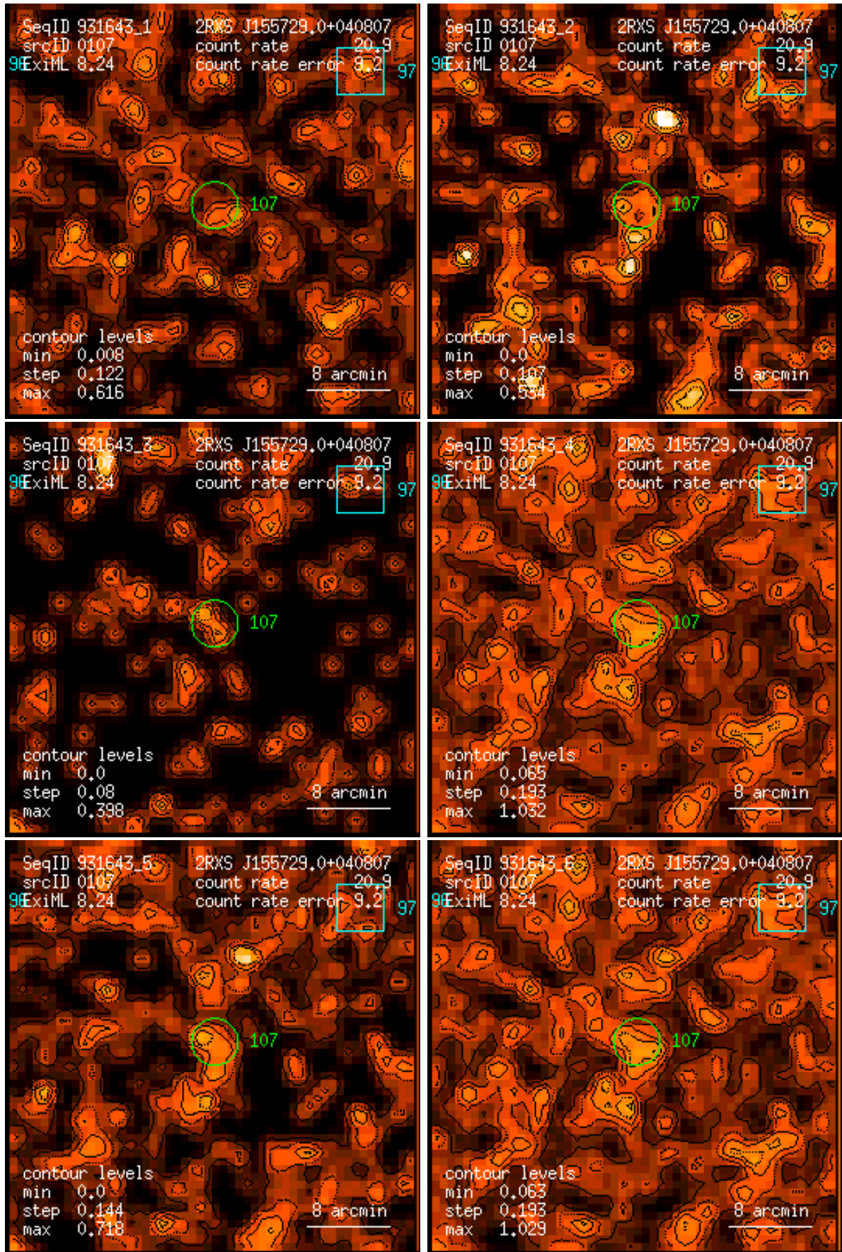
Figure 107: RASS 931643: detection 0107: band rate images, Gaussian filter: (1) PSPC channels 11 – 41, (2) 52 – 90, (3) 91 – 201, (4) 11 – 235, (5) 52 – 201, (6) 11 – 201. Broad band rates in counts/ks. Band rate contour levels in counts/ks/arcmin 2 .
