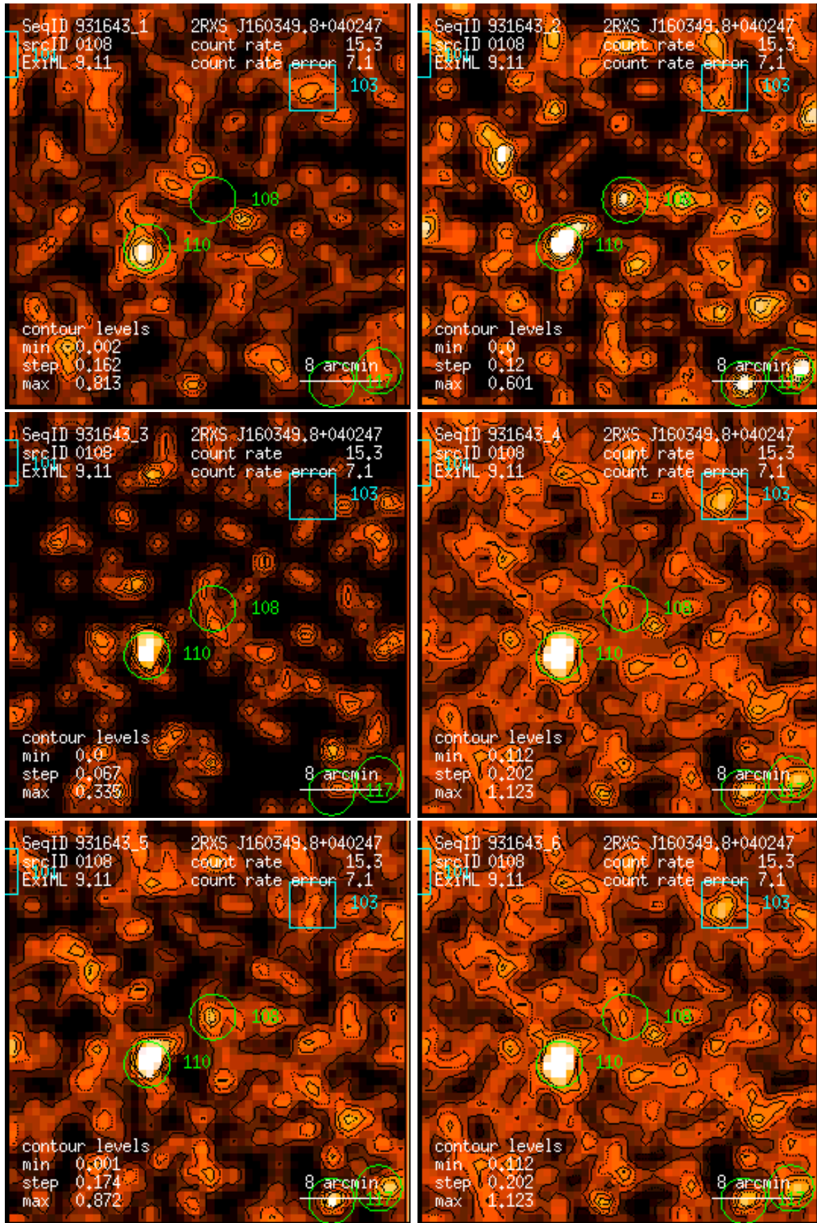
Figure 108: RASS 931643: detection 0108: band rate images, Gaussian filter: (1) PSPC channels 11 – 41, (2) 52 – 90, (3) 91 – 201, (4) 11 – 235, (5) 52 – 201, (6) 11 – 201. Broad band rates in counts/ks. Band rate contour levels in counts/ks/arcmin 2 .
