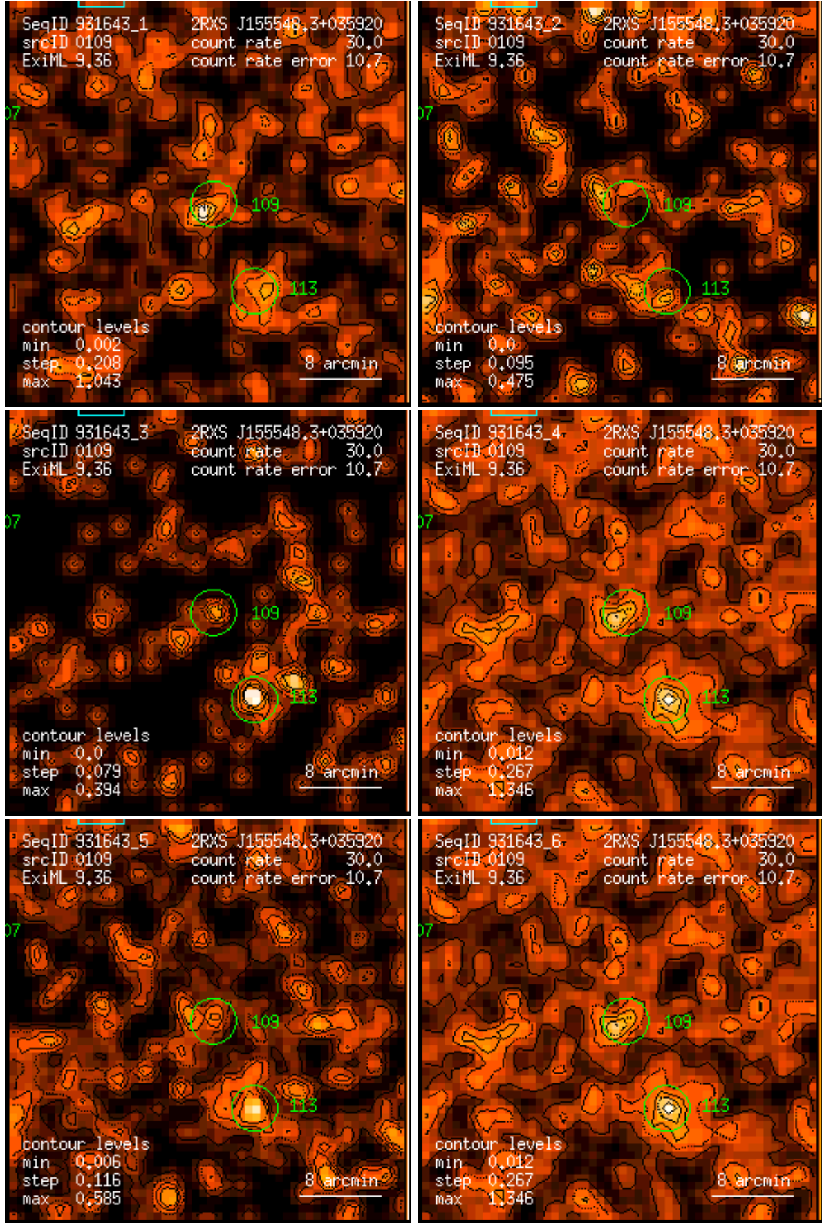
Figure 109: RASS 931643: detection 0109: band rate images, Gaussian filter: (1) PSPC channels 11 – 41, (2) 52 – 90, (3) 91 – 201, (4) 11 – 235, (5) 52 – 201, (6) 11 – 201. Broad band rates in counts/ks. Band rate contour levels in counts/ks/arcmin 2 .
