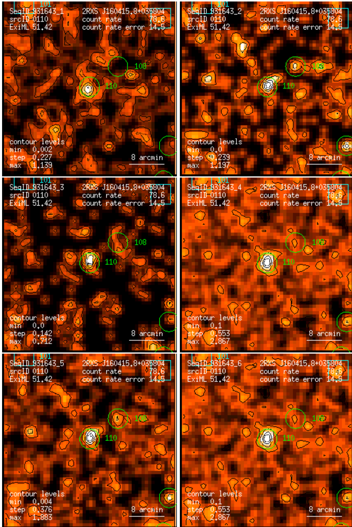
Figure 110: RASS 931643: detection 0110: band rate images, Gaussian filter: (1) PSPC channels 11 – 41, (2) 52 – 90, (3) 91 – 201, (4) 11 – 235, (5) 52 – 201, (6) 11 – 201. Broad band rates in counts/ks. Band rate contour levels in counts/ks/arcmin 2 .
