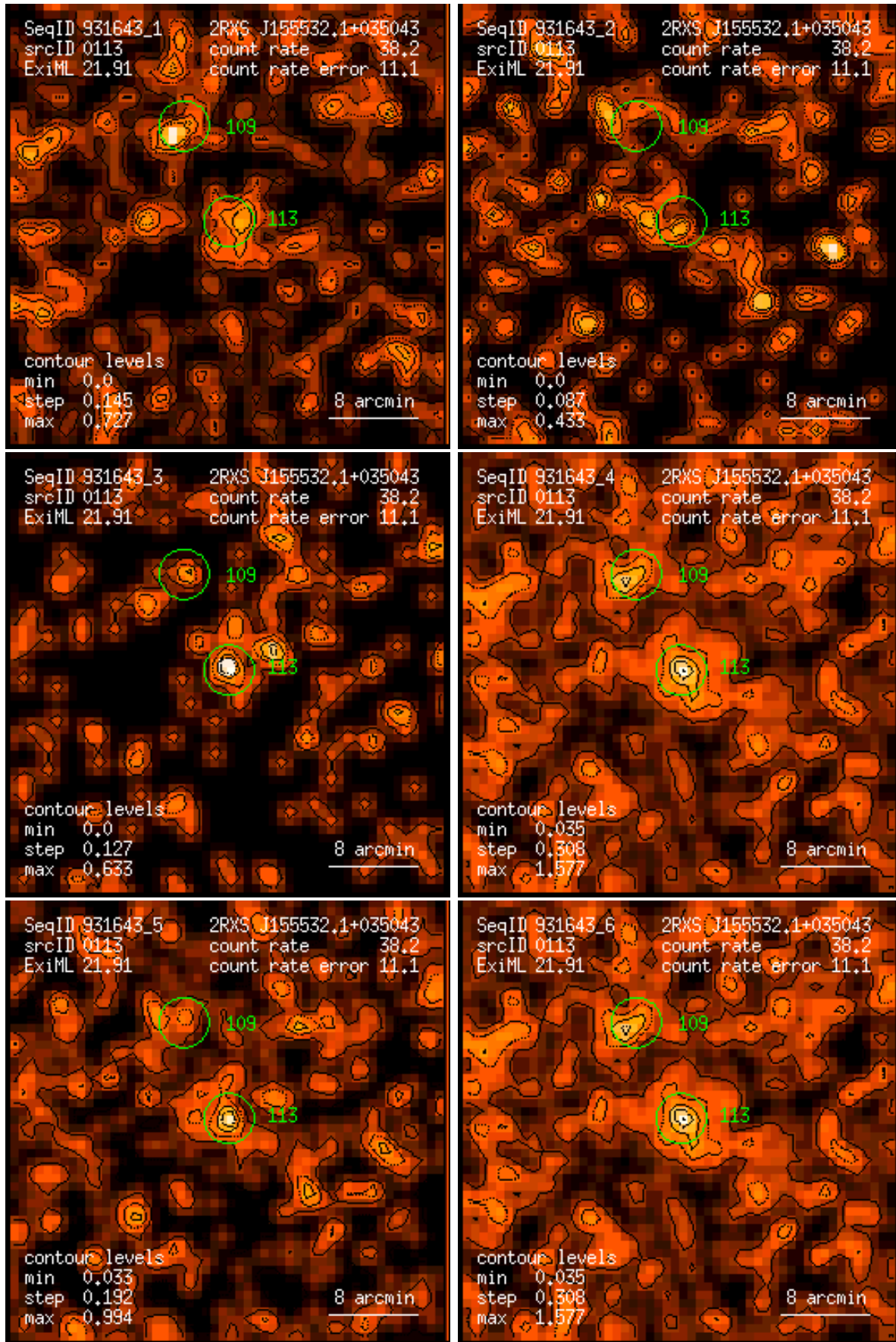
Figure 113: RASS 931643: detection 0113: band rate images, Gaussian filter: (1) PSPC channels 11 – 41, (2) 52 – 90, (3) 91 – 201, (4) 11 – 235, (5) 52 – 201, (6) 11 – 201. Broad band rates in counts/ks. Band rate contour levels in counts/ks/arcmin 2 .
