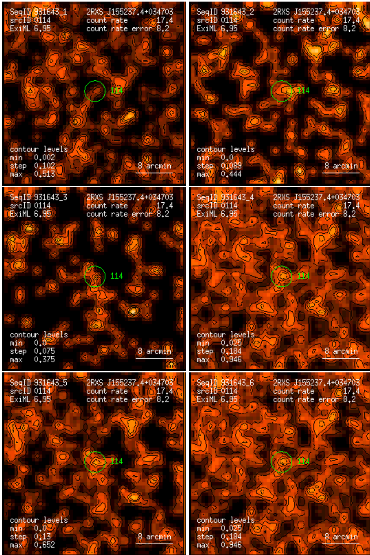
Figure 114: RASS 931643: detection 0114: band rate images, Gaussian filter: (1) PSPC channels 11 – 41, (2) 52 – 90, (3) 91 – 201, (4) 11 – 235, (5) 52 – 201, (6) 11 – 201. Broad band rates in counts/ks. Band rate contour levels in counts/ks/arcmin 2 .
