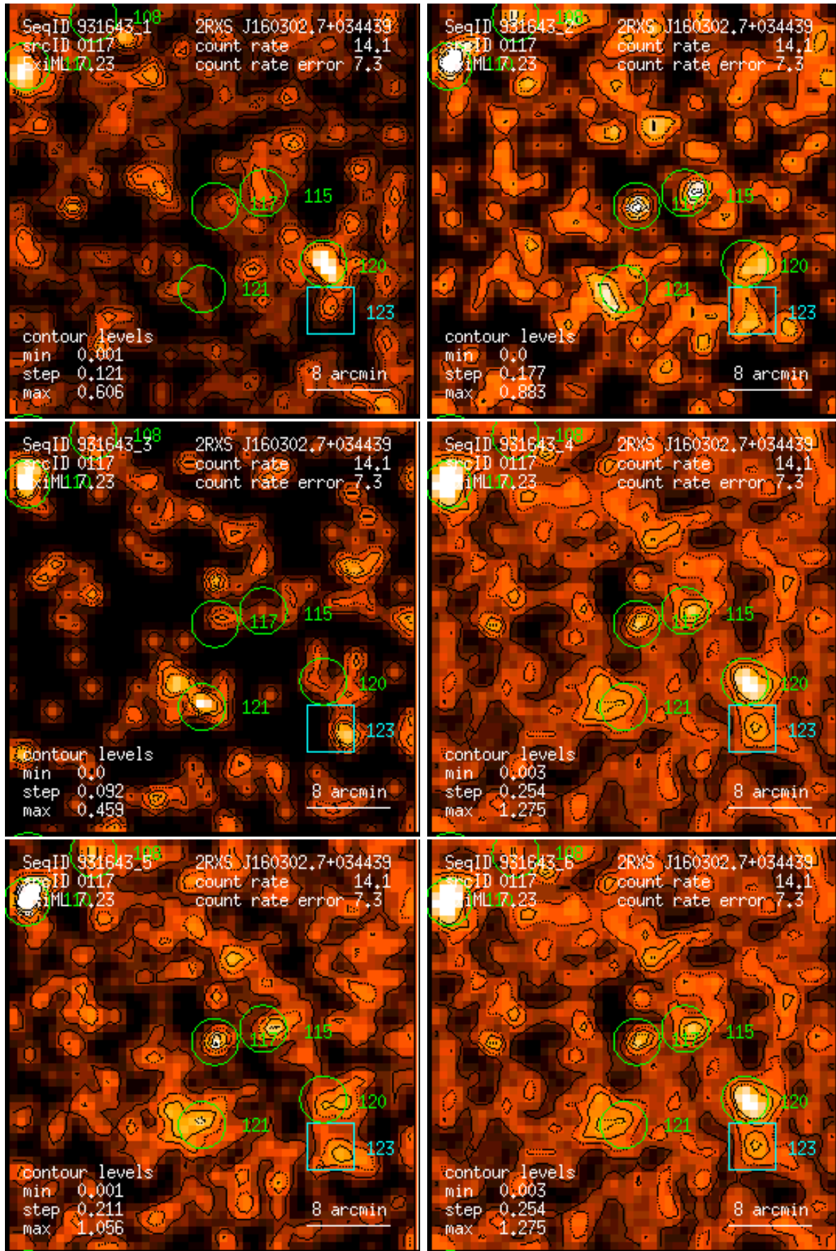
Figure 117: RASS 931643: detection 0117: band rate images, Gaussian filter: (1) PSPC channels 11 – 41, (2) 52 – 90, (3) 91 – 201, (4) 11 – 235, (5) 52 – 201, (6) 11 – 201. Broad band rates in counts/ks. Band rate contour levels in counts/ks/arcmin 2 .
