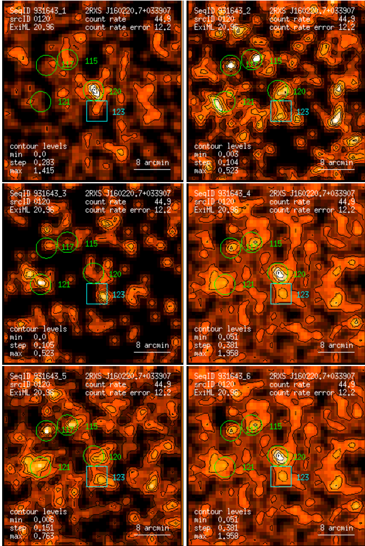
Figure 120: RASS 931643: detection 0120: band rate images, Gaussian filter: (1) PSPC channels 11 – 41, (2) 52 – 90, (3) 91 – 201, (4) 11 – 235, (5) 52 – 201, (6) 11 – 201. Broad band rates in counts/ks. Band rate contour levels in counts/ks/arcmin 2 .
