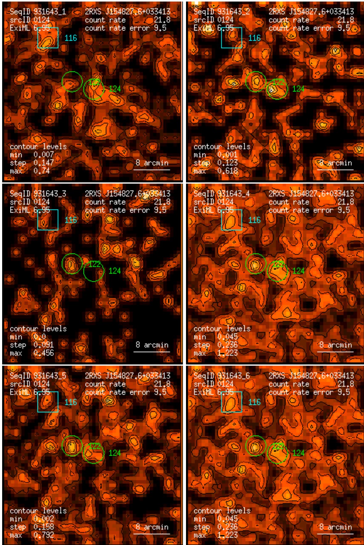
Figure 124: RASS 931643: detection 0124: band rate images, Gaussian filter: (1) PSPC channels 11 – 41, (2) 52 – 90, (3) 91 – 201, (4) 11 – 235, (5) 52 – 201, (6) 11 – 201. Broad band rates in counts/ks. Band rate contour levels in counts/ks/arcmin 2 .
