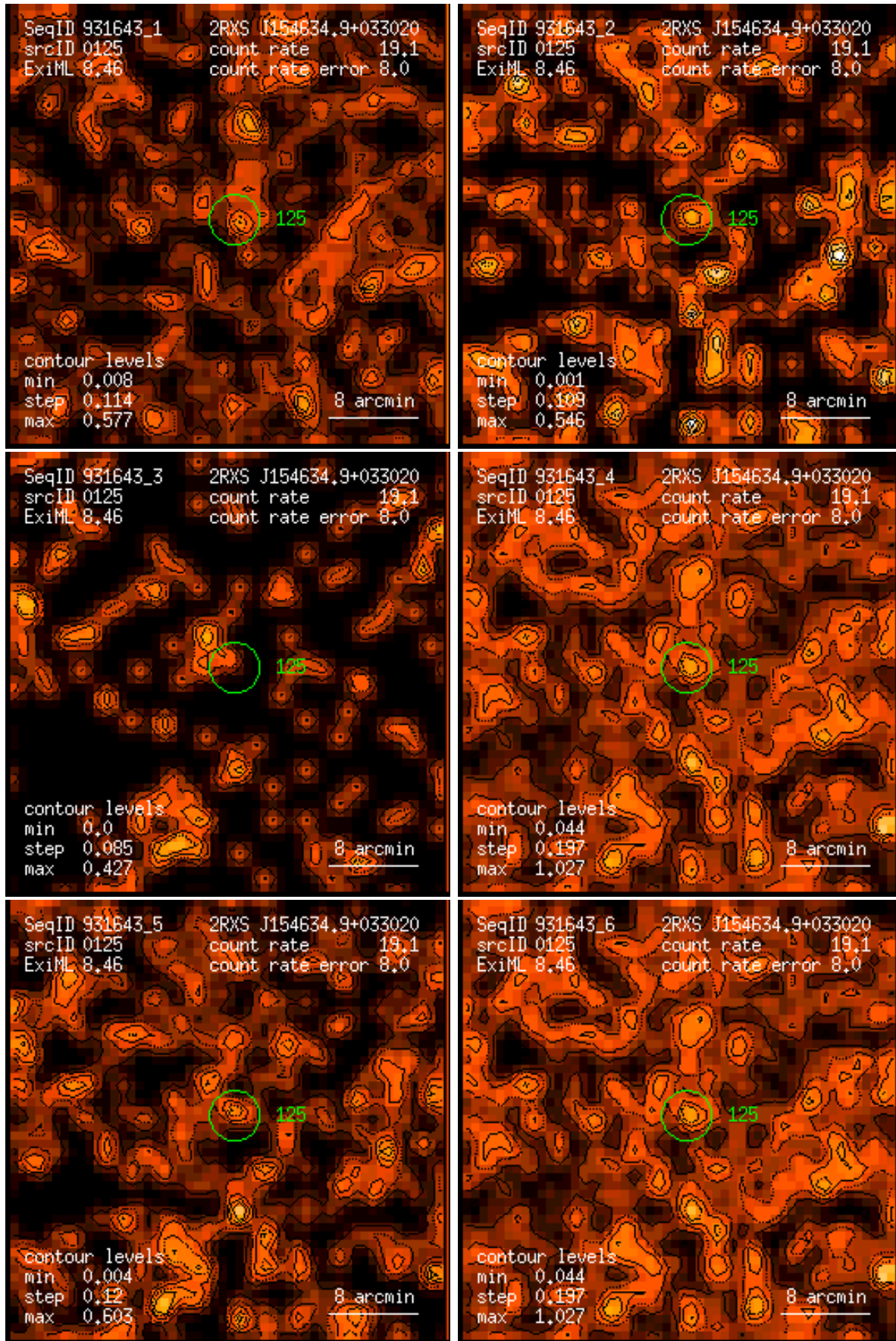
Figure 125: RASS 931643: detection 0125: band rate images, Gaussian filter: (1) PSPC channels 11 – 41, (2) 52 – 90, (3) 91 – 201, (4) 11 – 235, (5) 52 – 201, (6) 11 – 201. Broad band rates in counts/ks. Band rate contour levels in counts/ks/arcmin 2 .
