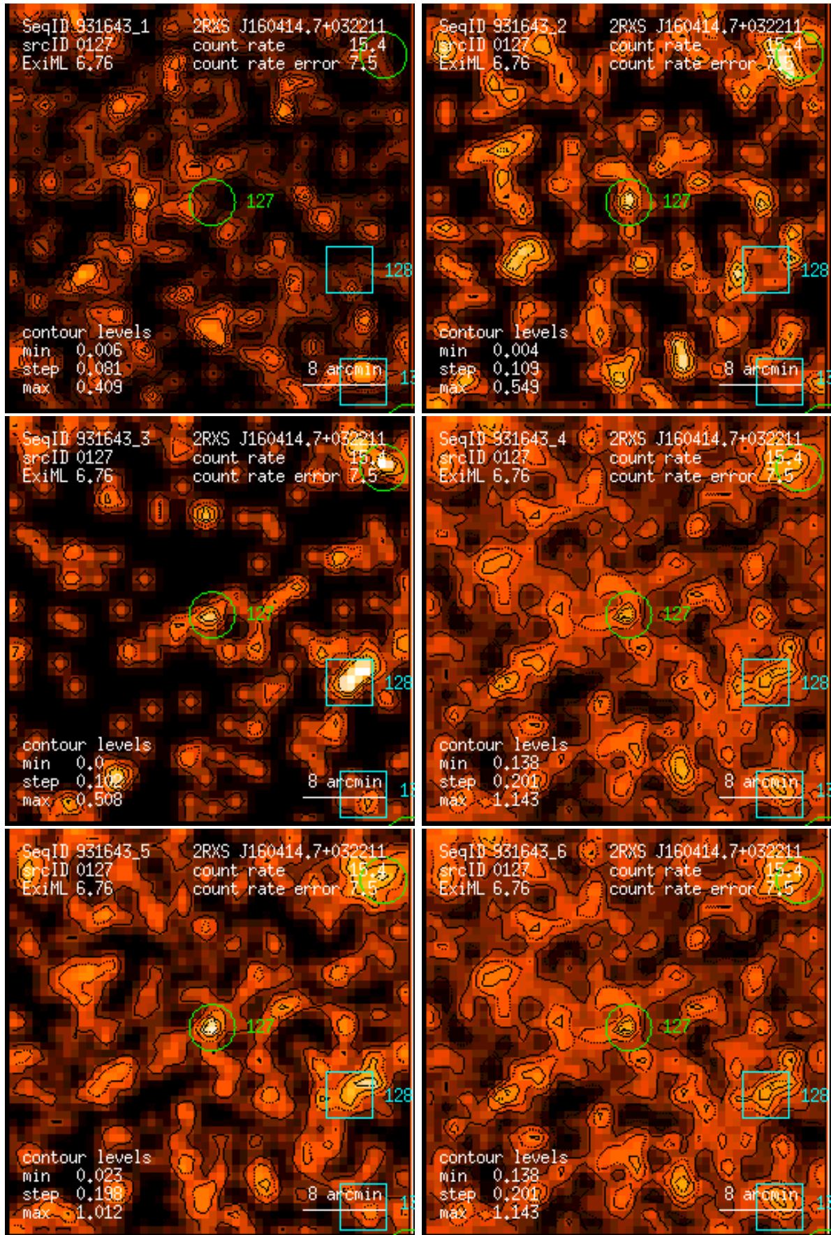
Figure 127: RASS 931643: detection 0127: band rate images, Gaussian filter: (1) PSPC channels 11 – 41, (2) 52 – 90, (3) 91 – 201, (4) 11 – 235, (5) 52 – 201, (6) 11 – 201. Broad band rates in counts/ks. Band rate contour levels in counts/ks/arcmin 2 .
