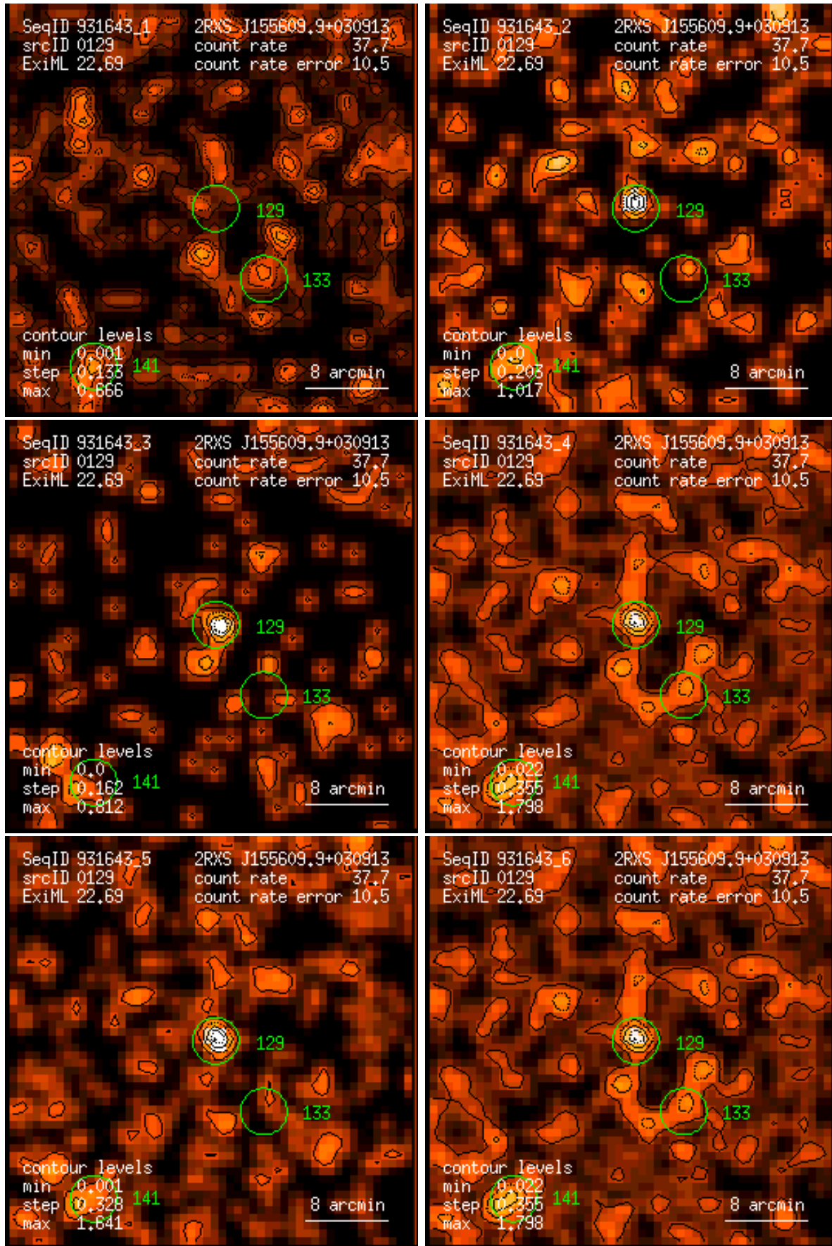
Figure 129: RASS 931643: detection 0129: band rate images, Gaussian filter: (1) PSPC channels 11 – 41, (2) 52 – 90, (3) 91 – 201, (4) 11 – 235, (5) 52 – 201, (6) 11 – 201. Broad band rates in counts/ks. Band rate contour levels in counts/ks/arcmin 2 .
