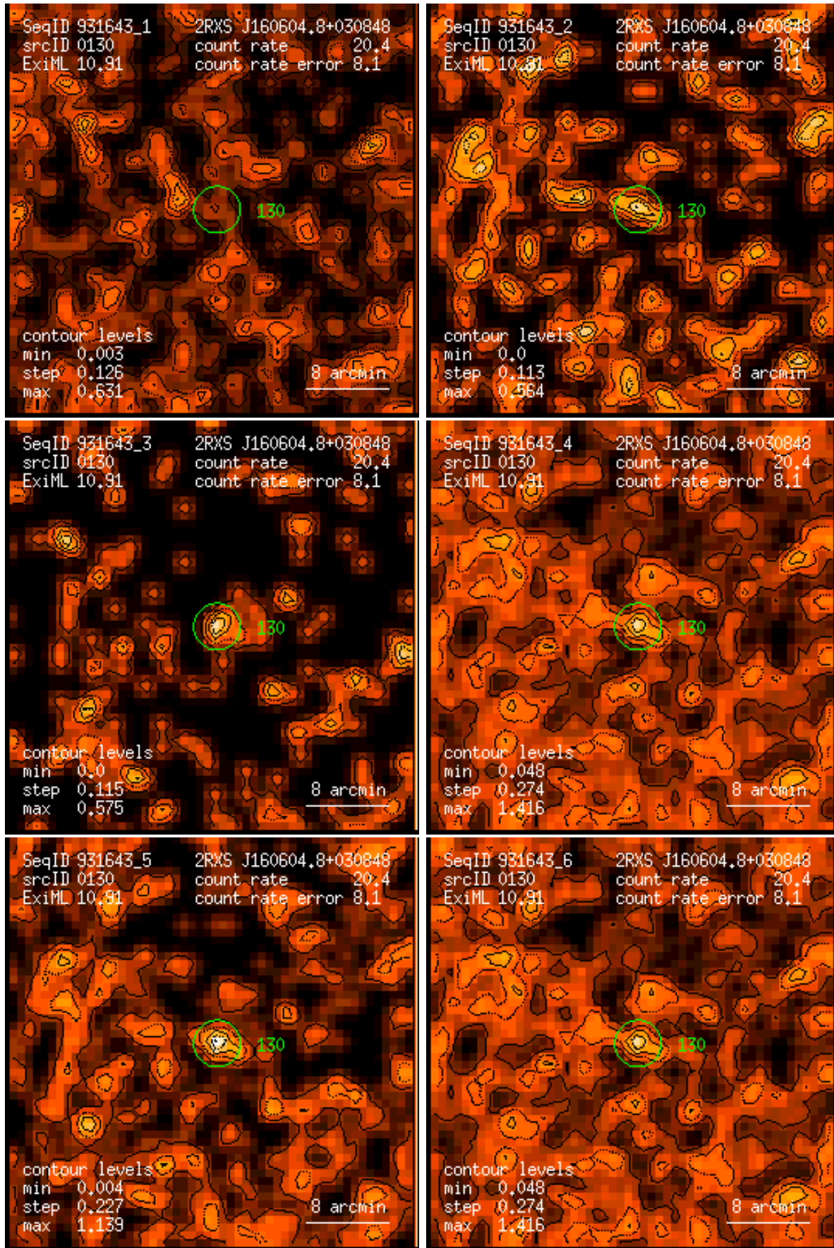
Figure 130: RASS 931643: detection 0130: band rate images, Gaussian filter: (1) PSPC channels 11 – 41, (2) 52 – 90, (3) 91 – 201, (4) 11 – 235, (5) 52 – 201, (6) 11 – 201. Broad band rates in counts/ks. Band rate contour levels in counts/ks/arcmin 2 .
