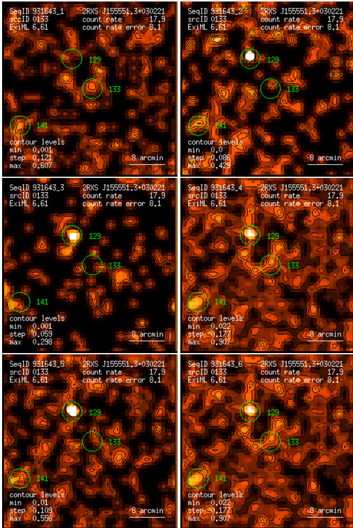
Figure 133: RASS 931643: detection 0133: band rate images, Gaussian filter: (1) PSPC channels 11 – 41, (2) 52 – 90, (3) 91 – 201, (4) 11 – 235, (5) 52 – 201, (6) 11 – 201. Broad band rates in counts/ks. Band rate contour levels in counts/ks/arcmin 2 .
